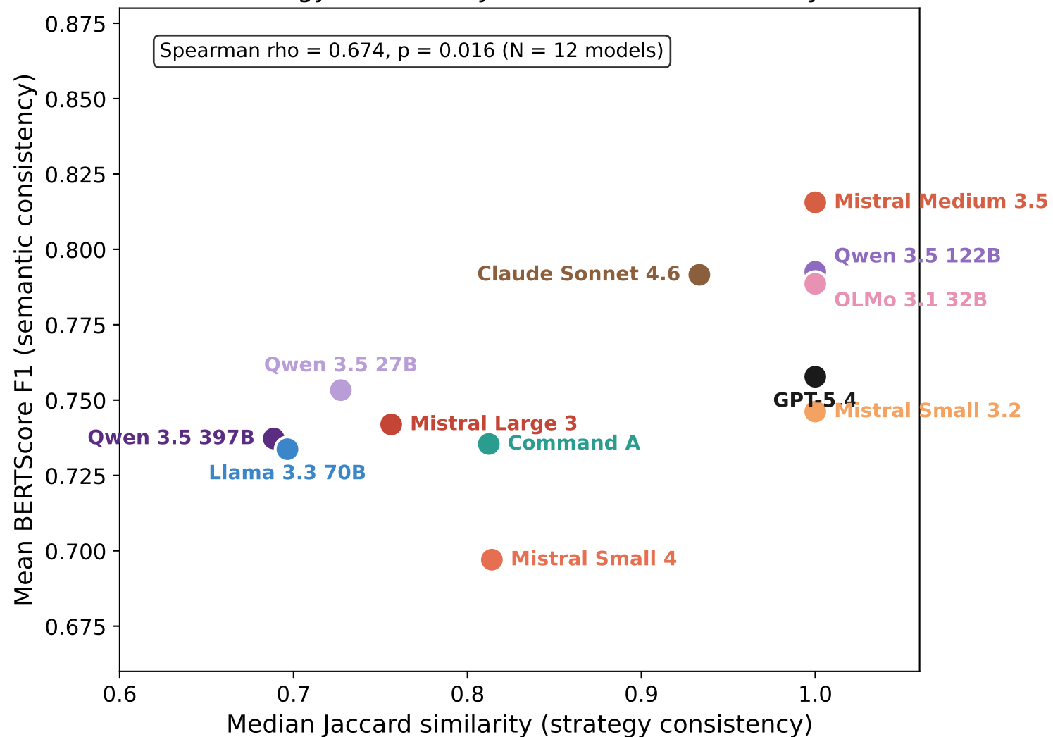
Strategy consistency vs semantic consistency
