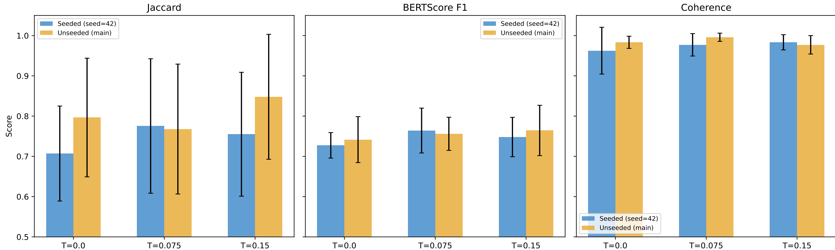
Mistral Large 3: Seeded vs Unseeded (20 trials, seed=42)
