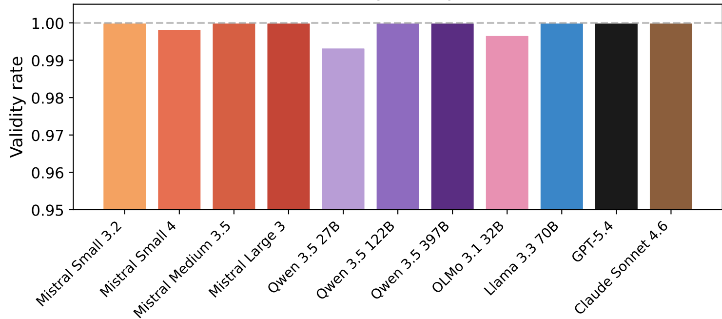
Plan validity rate by model
