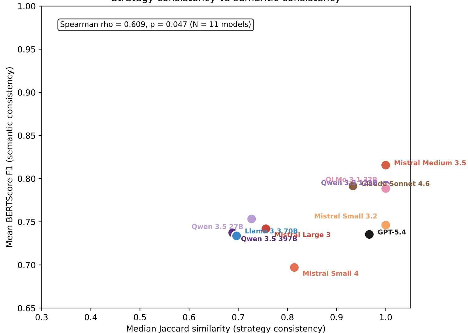
Strategy consistency vs semantic consistency
