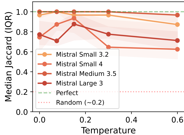
Mistral family
