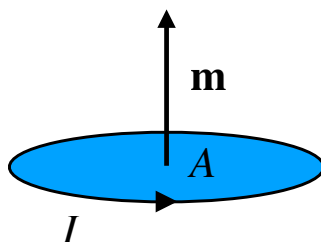
Figure 6: A magnetic dipole moment \mathbf{m} is generated by a current loop. The direction of \mathbf{m} is given by the right-hand rule.
