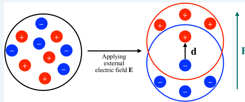
Figure 4: When an electric field is applied, the positive charges move in the direction of \mathbf{E} while the negative charges move in the opposite direction. As a result, the spheres are shifted against each other.
