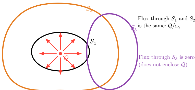
Figure 1: The flux through S_1 and S_2 is the same ( = Q/\varepsilon_0 ), since both enclose Q . The flux through S_3 is zero: as much flux enters V_3 as leaves it, since S_3 does not enclose the charge.
