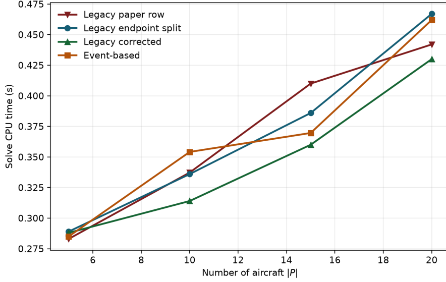
Figure 6: Solver CPU time versus fleet size on the heavy A-only suite.
