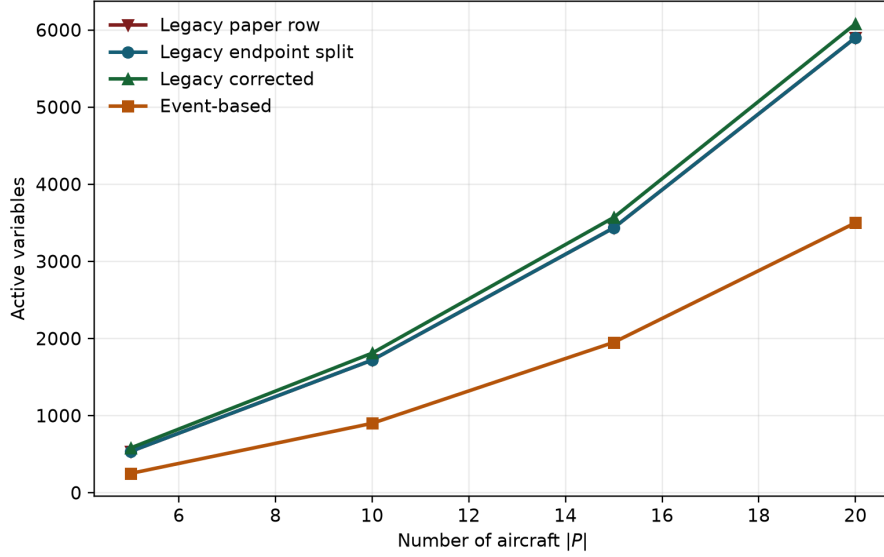
Figure 4: Active model variables versus fleet size on the heavy A-only suite.
