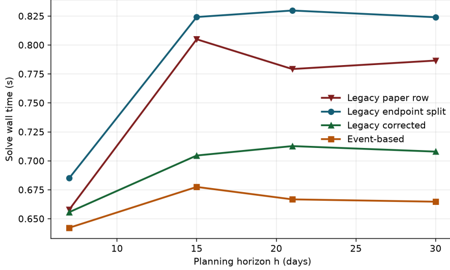
Figure 2: A-only solve wall time versus planning horizon for the four-method comparison.
