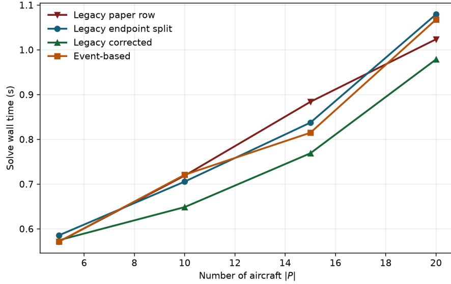
Figure 7: Solver wall time versus fleet size on the heavy A-only suite.
