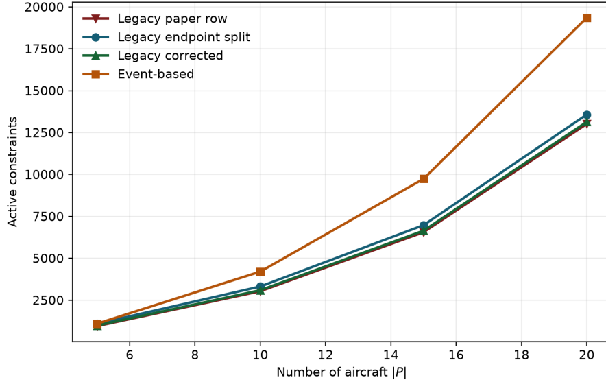
Figure 5: Active model constraints versus fleet size on the heavy A-only suite.
