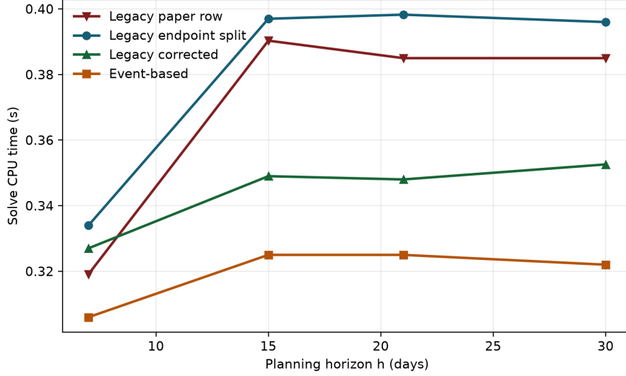
Figure 3: A-only solve CPU time versus planning horizon for the four-method comparison.
