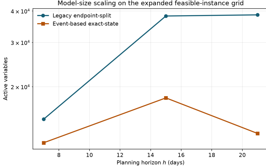
Figure 2: Active variable count versus horizon on the same feasible heavy instances. The event formulation uses fewer variables in these three cases.
