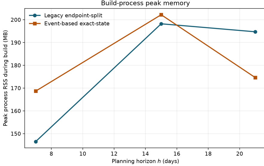
Figure 5: Peak resident set size of the Python process during model construction on the heavy instances. Measurements use psutil ; this is a build-memory measurement, not peak memory of the external MILP solver process.
