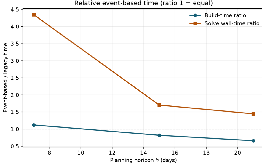
Figure 4: Relative event-based time on the objective-matched heavy instances. A ratio below one means the event formulation is faster; a ratio above one means it is slower. Build time can decrease at longer horizons, but solved wall time remains above the legacy value in every tested case.
