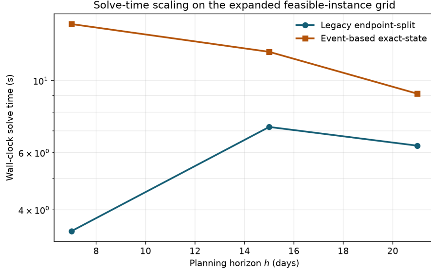
Figure 1: Wall-clock solve time versus horizon on objective-matched feasible heavy instances. The event formulation is slower on this sample, although both formulations return the same optimum.
