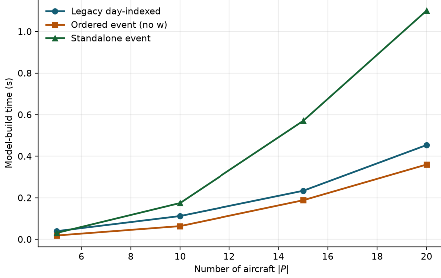
Figure 3: Model-build wall time versus fleet size for the latest ordered no- w formulation, legacy model, and standalone event model.
