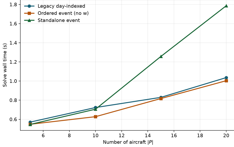
Figure 4: Solve wall time versus fleet size for the latest ordered no- w formulation, legacy model, and standalone event model. All runs are optimal and objective-matched.
