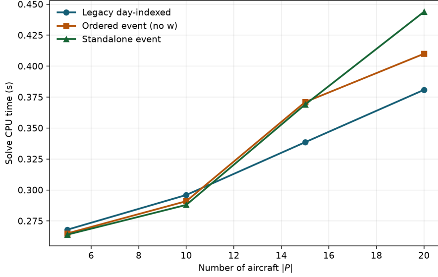
Figure 5: Solve CPU time versus fleet size for the latest ordered no- w formulation, legacy model, and standalone event model. All runs are optimal and objective-matched.
