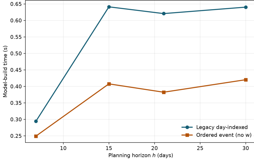
Figure 8: Model-build wall time versus planning horizon for legacy and ordered no- w formulations at fixed fleet size ( |P| = 10 ).
