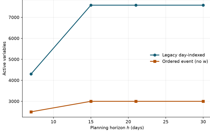
Figure 6: Active variable count versus planning horizon for legacy and ordered no- w formulations at fixed fleet size ( |P| = 10 ).
