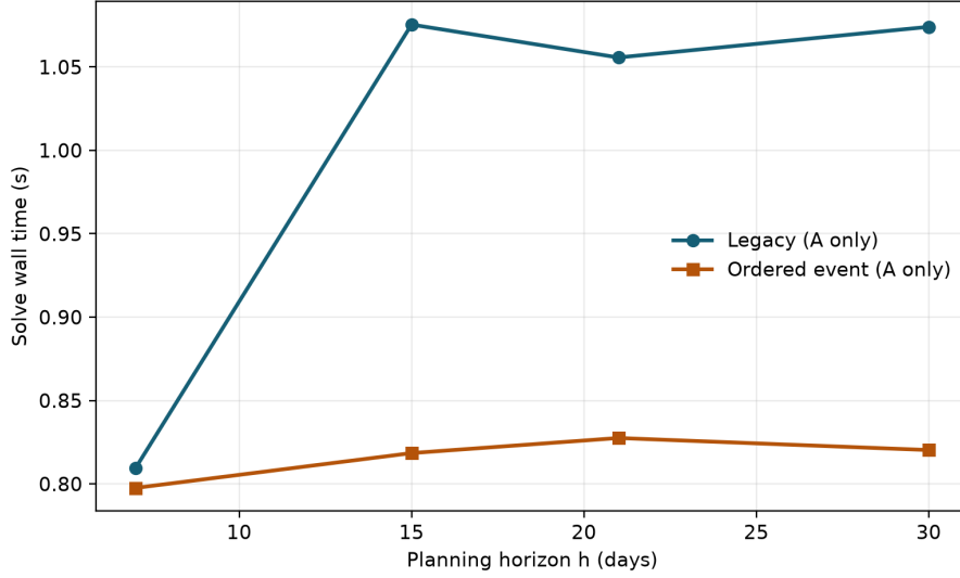
Figure 10: A-only solve wall time versus planning horizon for legacy and ordered A-event formulations.
