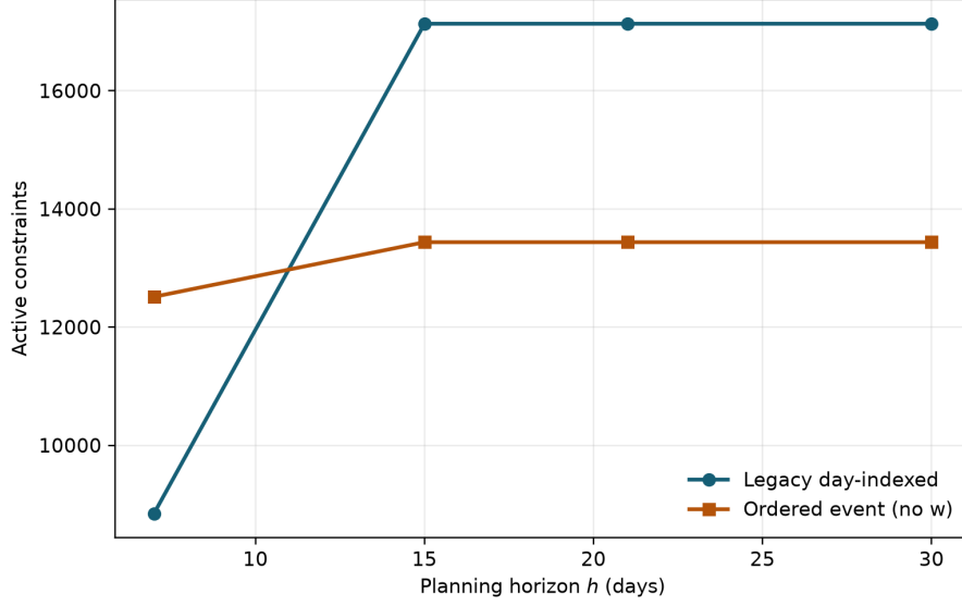
Figure 7: Active constraint count versus planning horizon for legacy and ordered no- w formulations at fixed fleet size ( |P| = 10 ).
