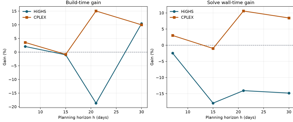
Figure 13: Solver-specific gains of the clique+tight ordered profile relative to pair-wise+coarse across horizon lengths. Positive values mean faster performance for clique+tight . Left: build-time gain. Right: solve wall-time gain.
