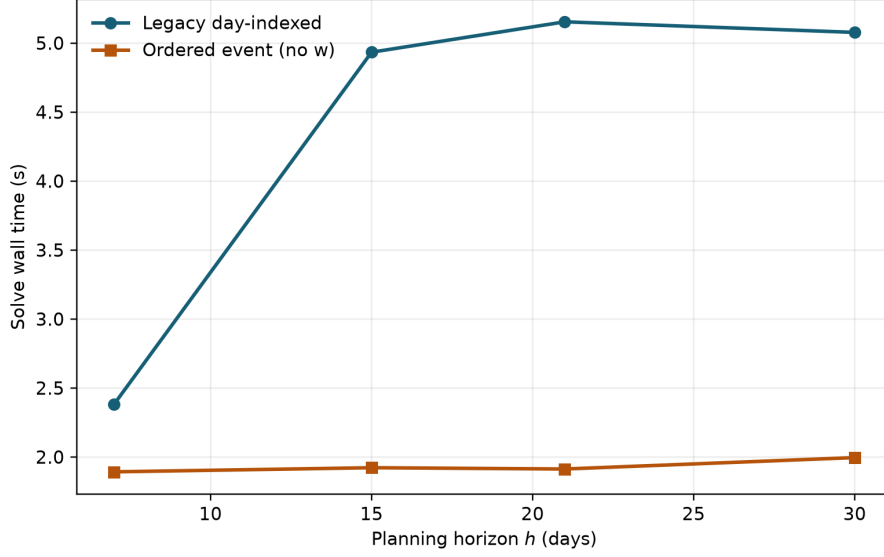
Figure 9: Solve wall time versus planning horizon for legacy and ordered no- w formulations at fixed fleet size ( |P| = 10 ).
