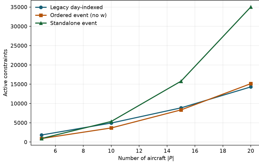
Figure 2: Active constraint count versus fleet size for the latest ordered no- w formulation, legacy model, and standalone event model.
