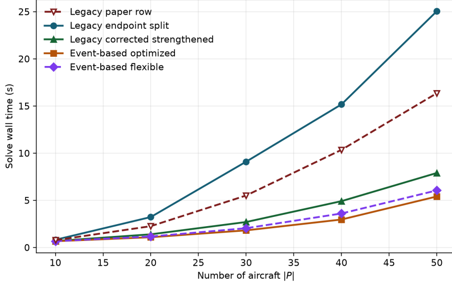
Figure 6: Solver wall time versus fleet size at H = 30 in the extended five-method A-only suite.
