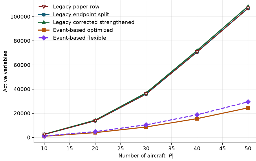
Figure 3: Active model variables versus fleet size at H = 30 in the extended five-method A-only suite.
