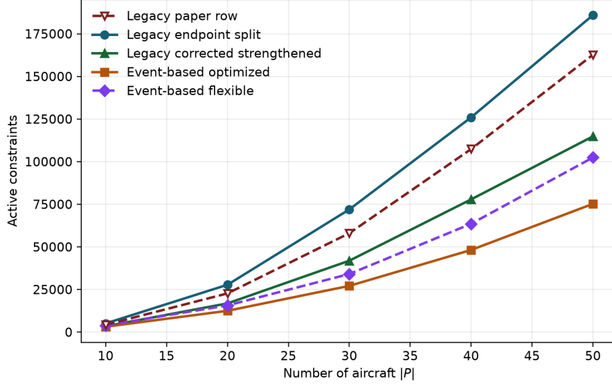
Figure 4: Active model constraints versus fleet size at H = 30 in the extended five-method A-only suite.
