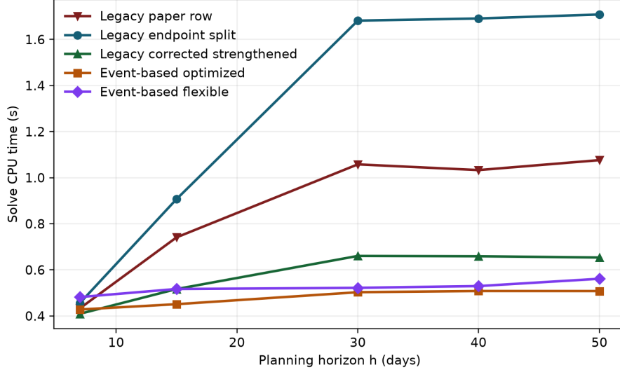
Figure 2: A-only solve CPU time versus planning horizon for the five-method comparison at |P| = 20 in the extended suite.
