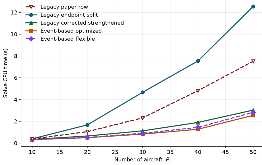
Figure 5: Solver CPU time versus fleet size at H = 30 in the extended five-method A-only suite.
