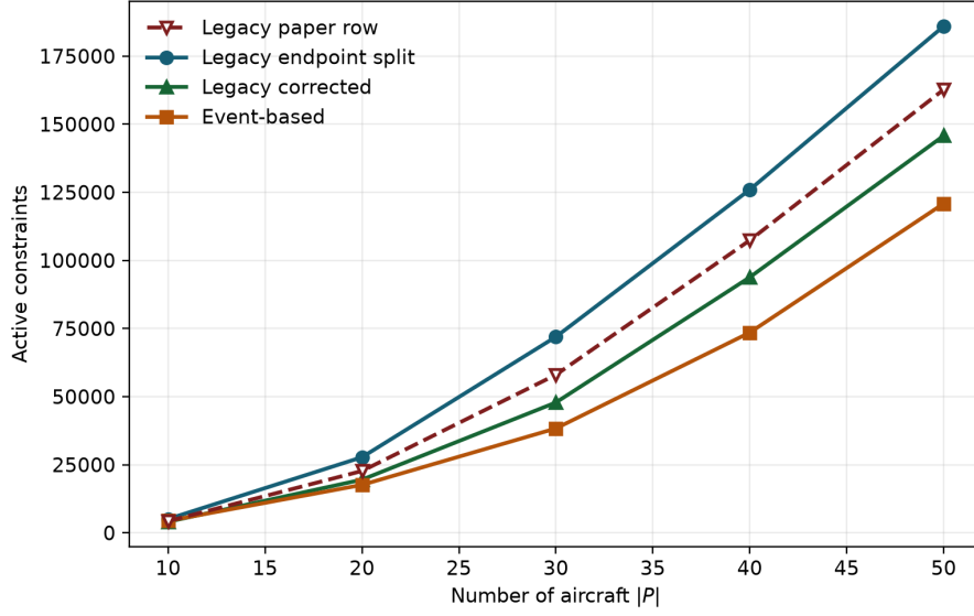
Figure 5: Active model constraints versus fleet size at H = 30 in the extended four-method A-only suite.
