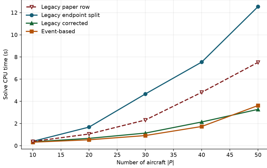
Figure 6: Solver CPU time versus fleet size at H = 30 in the extended four-method A-only suite.
