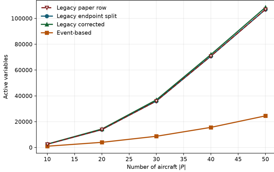
Figure 4: Active model variables versus fleet size at H = 30 in the extended four-method A-only suite.
