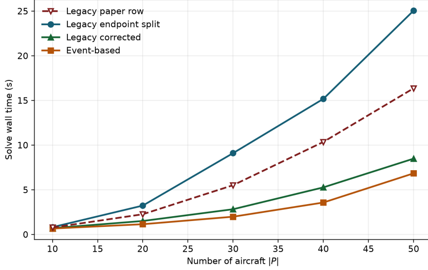
Figure 7: Solver wall time versus fleet size at H = 30 in the extended four-method A-only suite.
