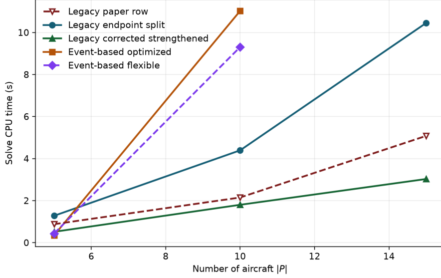
Figure 5: A-only solve CPU time versus fleet size at observed horizon H = 30 . Only optimal runs are plotted.
