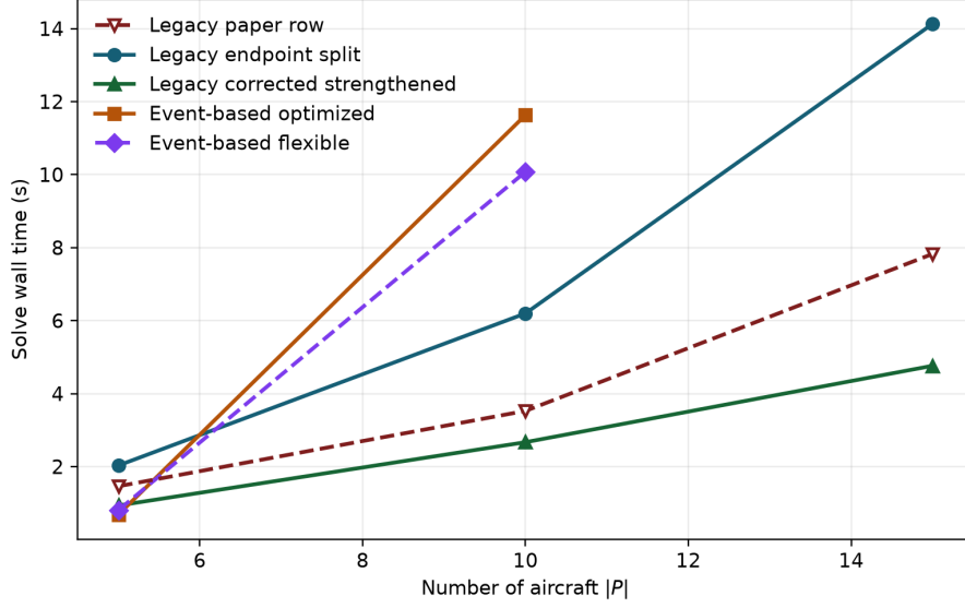
Figure 6: A-only solve wall time versus fleet size at observed horizon H = 30 . Only optimal runs are plotted.
