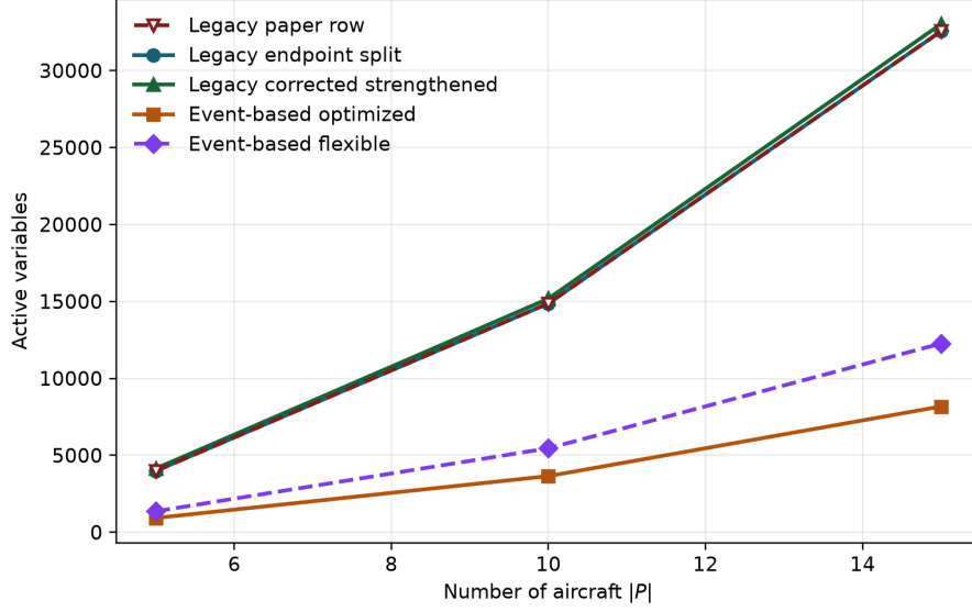
Figure 3: Active Pyomo variables versus fleet size at observed horizon H = 30 .
