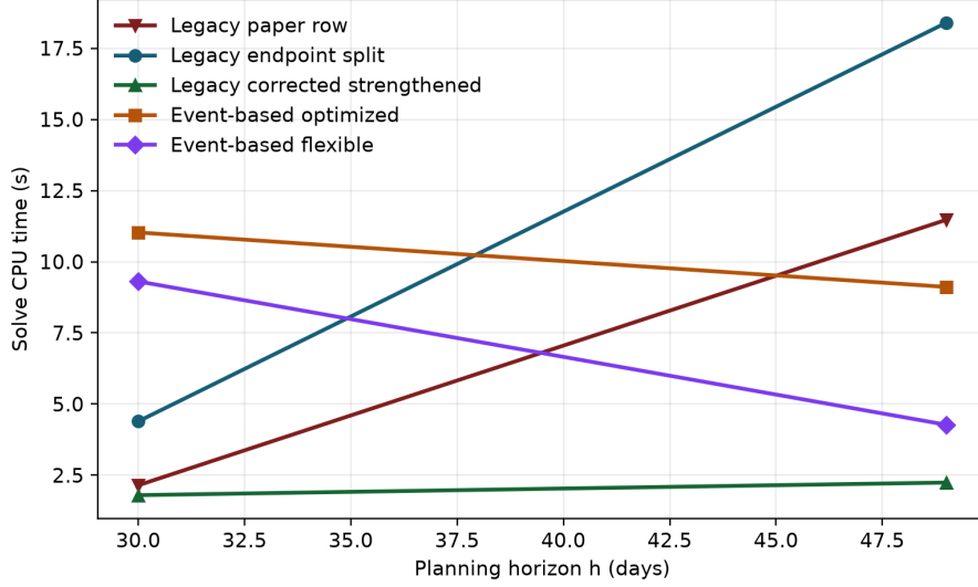
Figure 2: A-only solve CPU time versus observed horizon for |P| = 10 . Only optimal runs are plotted.
