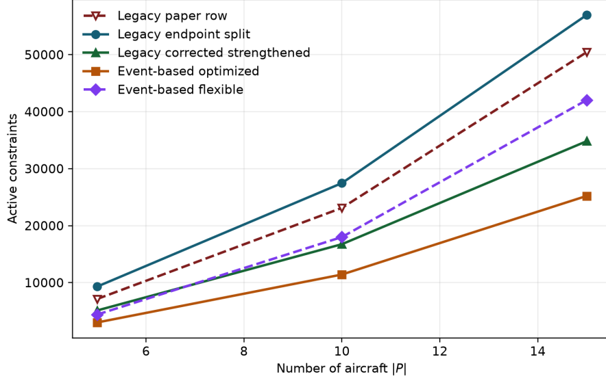
Figure 4: Active Pyomo constraints versus fleet size at observed horizon H = 30 .
