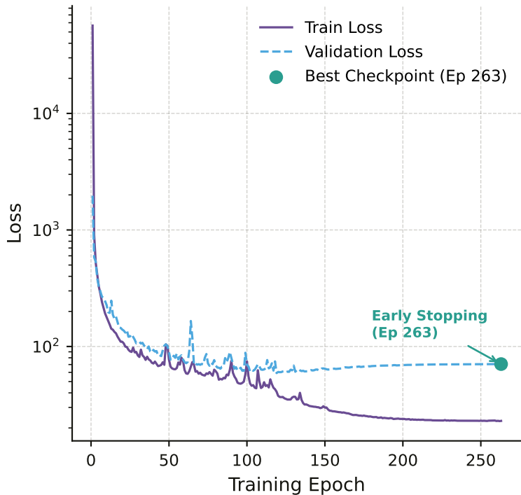
PaiNN Pre-AL Fine-Tuning (500 Epochs)
