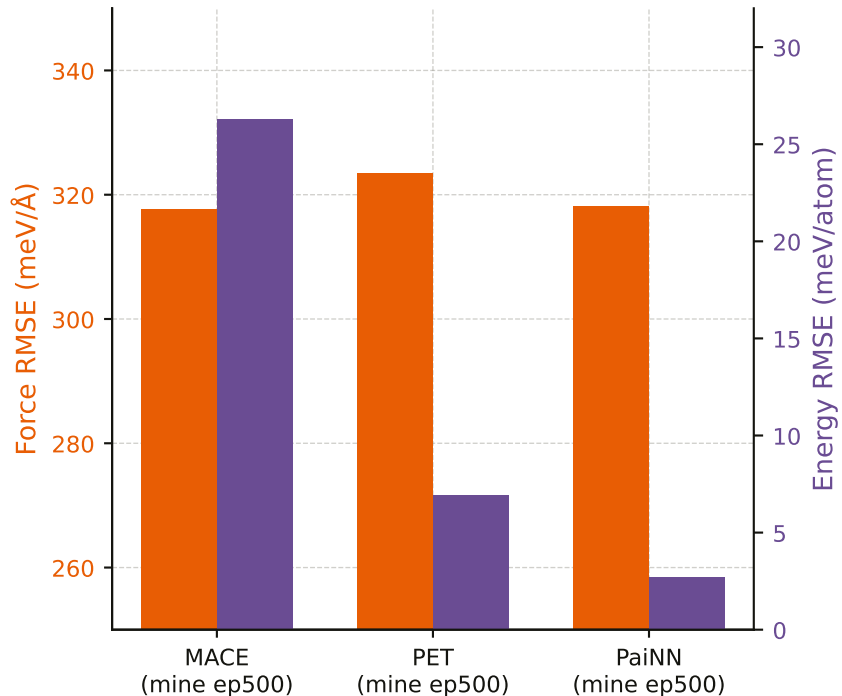
MLIP Pre-AL Test Set Errors (Mine Data)
