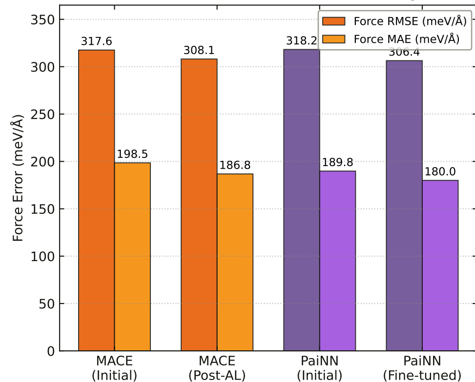
(a) Pre-AL Baseline vs. Post-AL Model Convergence
