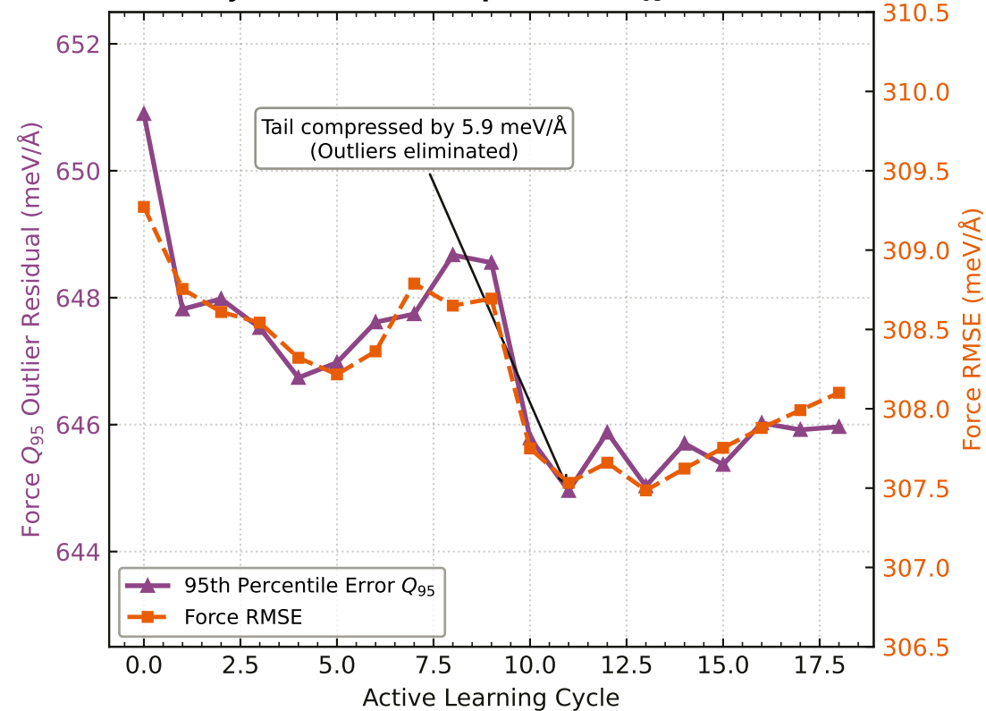
(c) Heavy-Tail Outlier Compression ( Q_{95} & RMSE)
