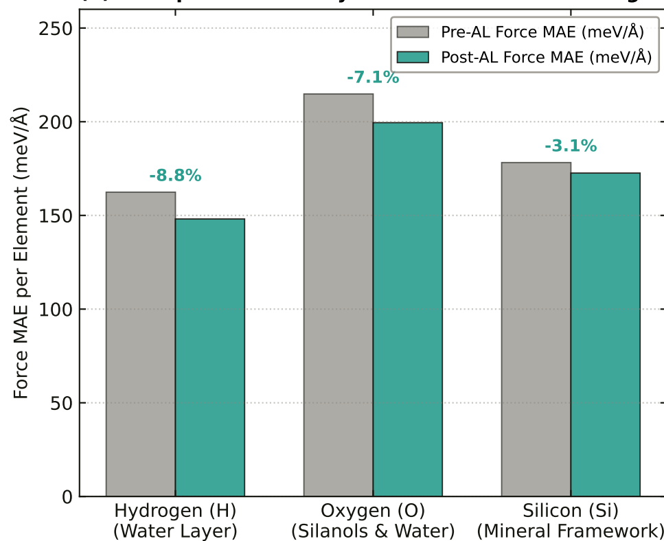
(d) Per-Species Accuracy Gain from Active Learning
