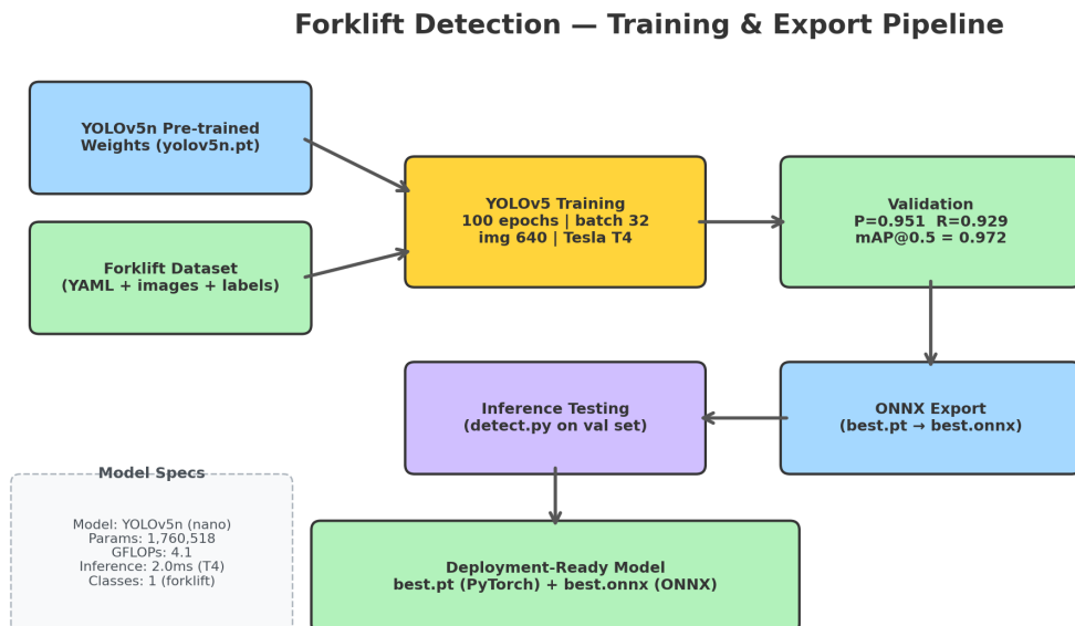
Figure 3.7: Forklift detection model training and export pipeline.
