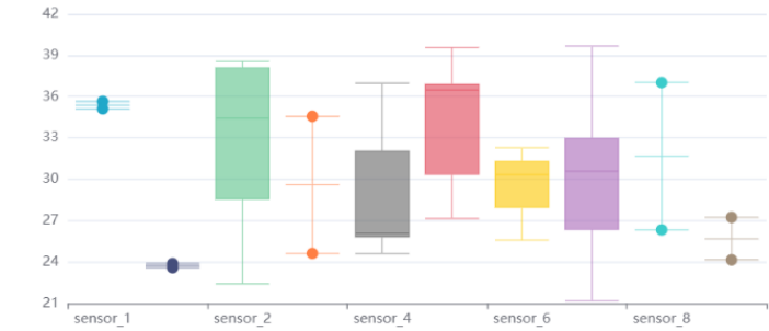
Distribution of temperature measurements by device
