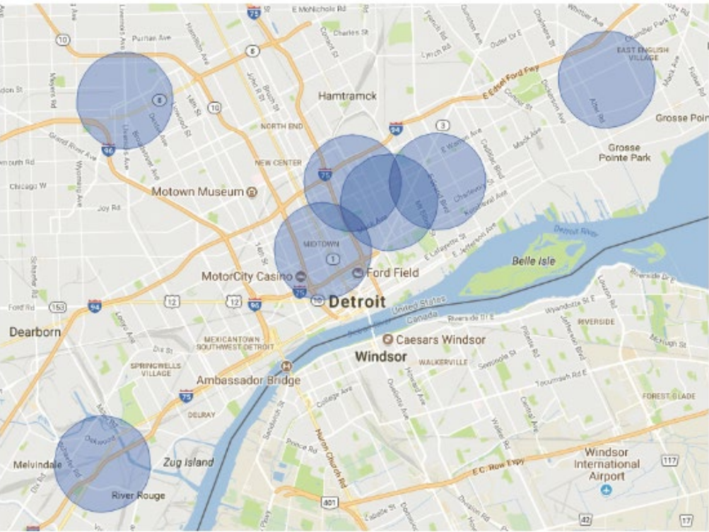
Figure 2 Location of DCTP Wireless Mesh Networks.
