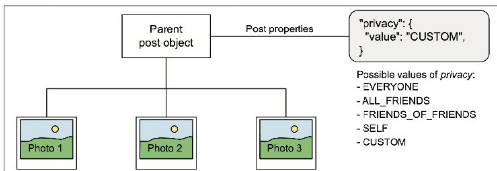
Figure 5. In Facebook's API, photo objects themselves do not have a privacy field, so Bridgy checks the privacy field of their parent post.
