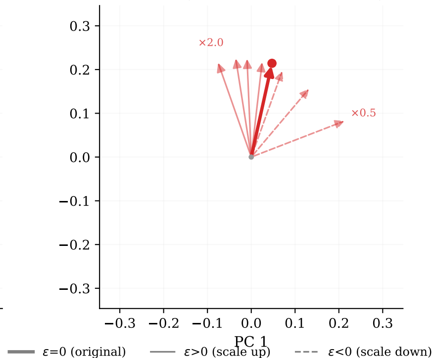
GELU (18.8° total rotation)
