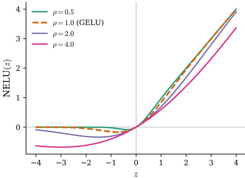
(a) NELU activation shape
