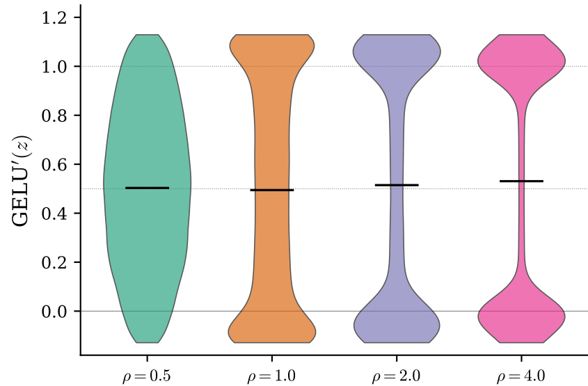
(c) GELU derivative, z \sim \mathcal{N}(0, \rho^2)
