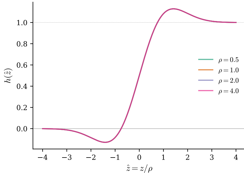
(b) NELU derivative (all \rho collapse)
