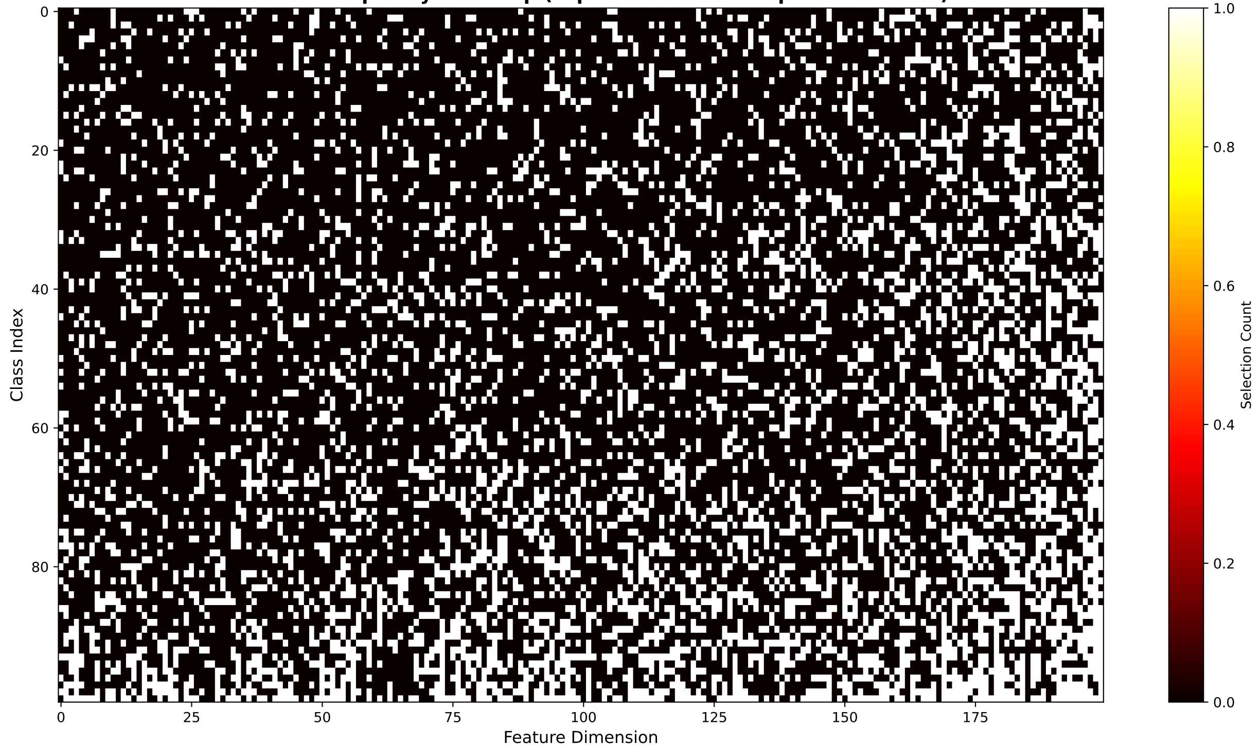
Selection Frequency Heatmap (Top 100 Classes × Top 200 Features)
