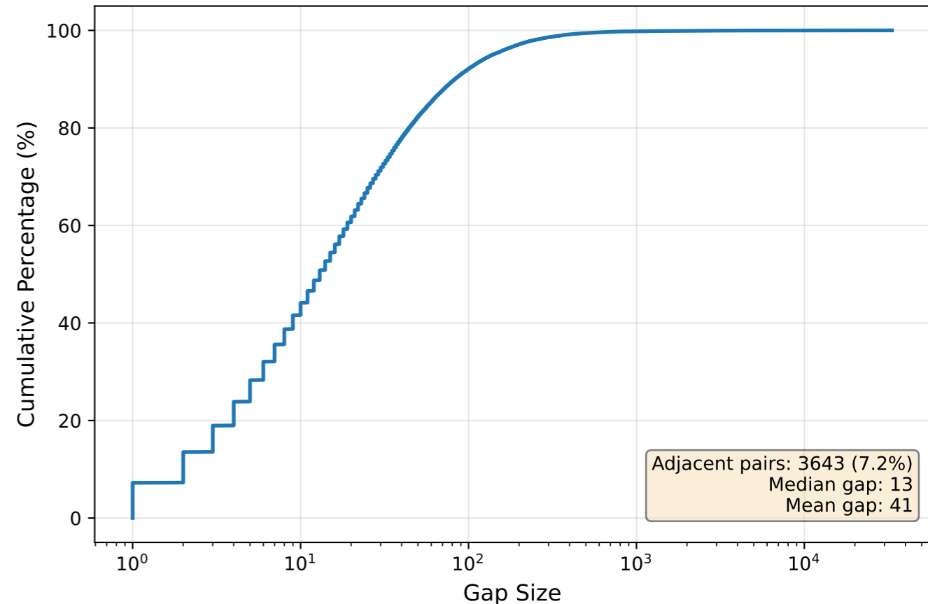
Cumulative Gap Distribution
