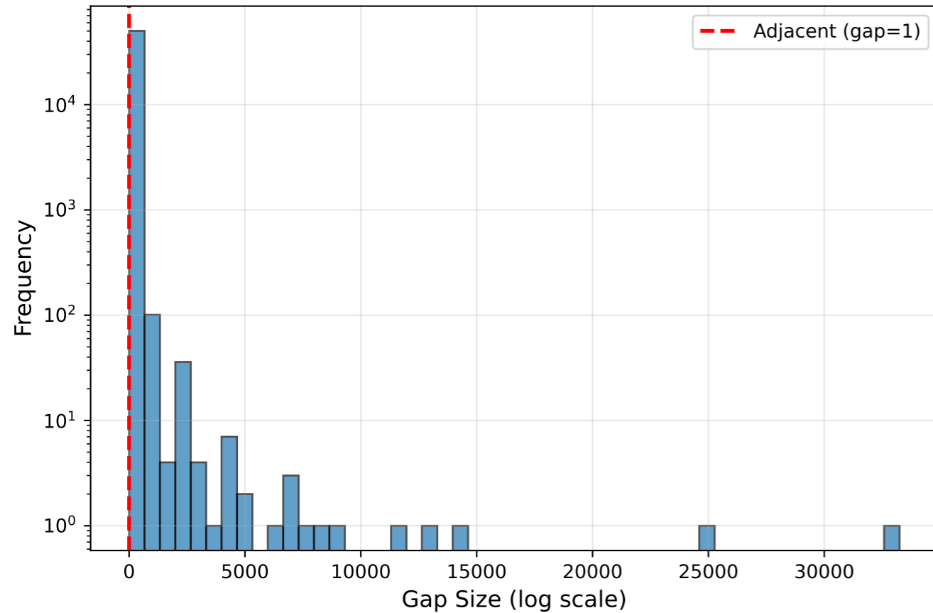
Distribution of Gaps Between Selected Indices
