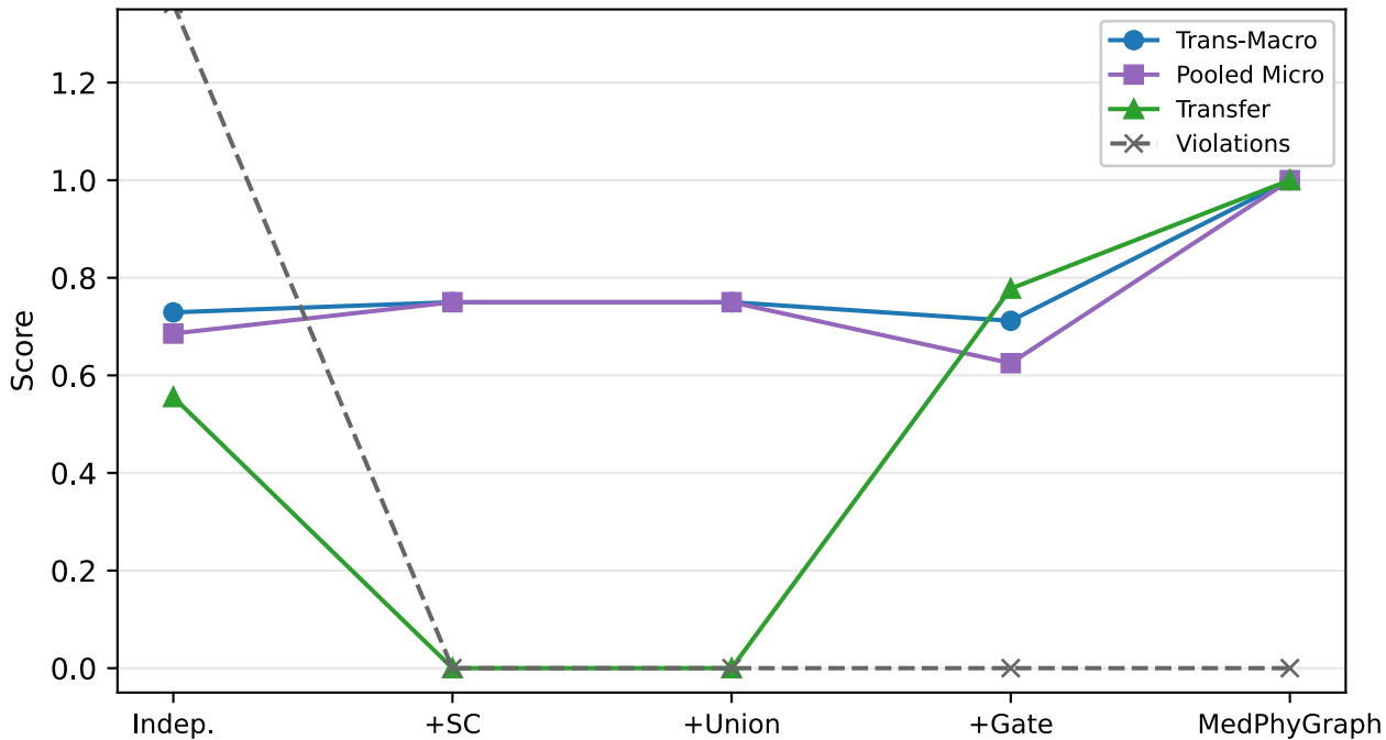
Refinement ablation (Isaac for Healthcare)
