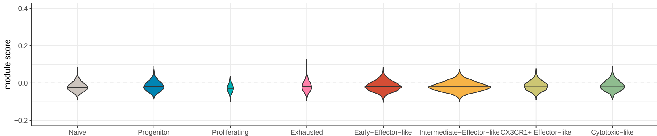
Genes with more accessible regions in H1-cKO Tprog
