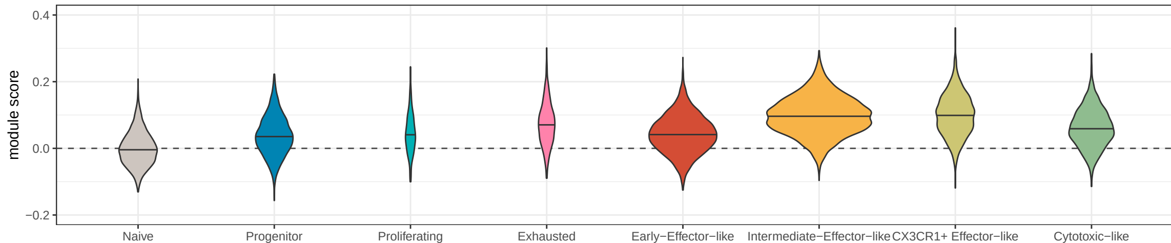
Genes with more accessible regions in WT Tprog
