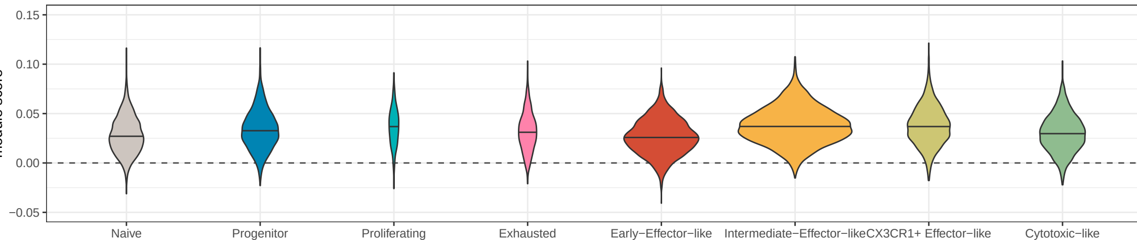
Genes with more accessible regions in WT nonTprog
