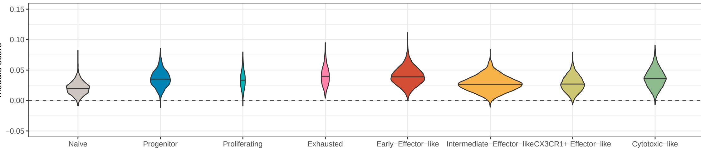
Genes with more accessible regions in H1-cKO nonTprog
