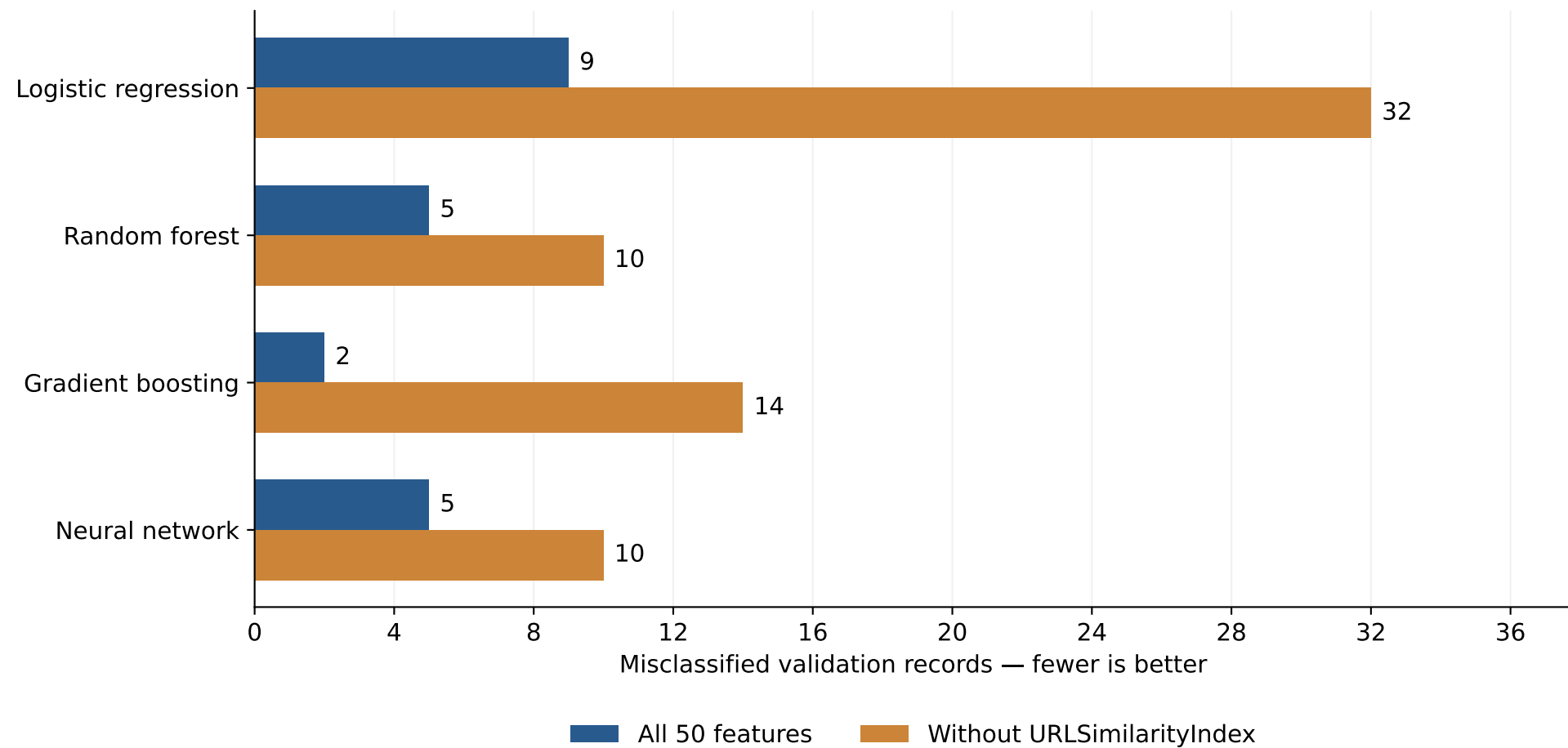
Effect of removing URLSimilarityIndex Same 45,028 validation records | Training seed 42
