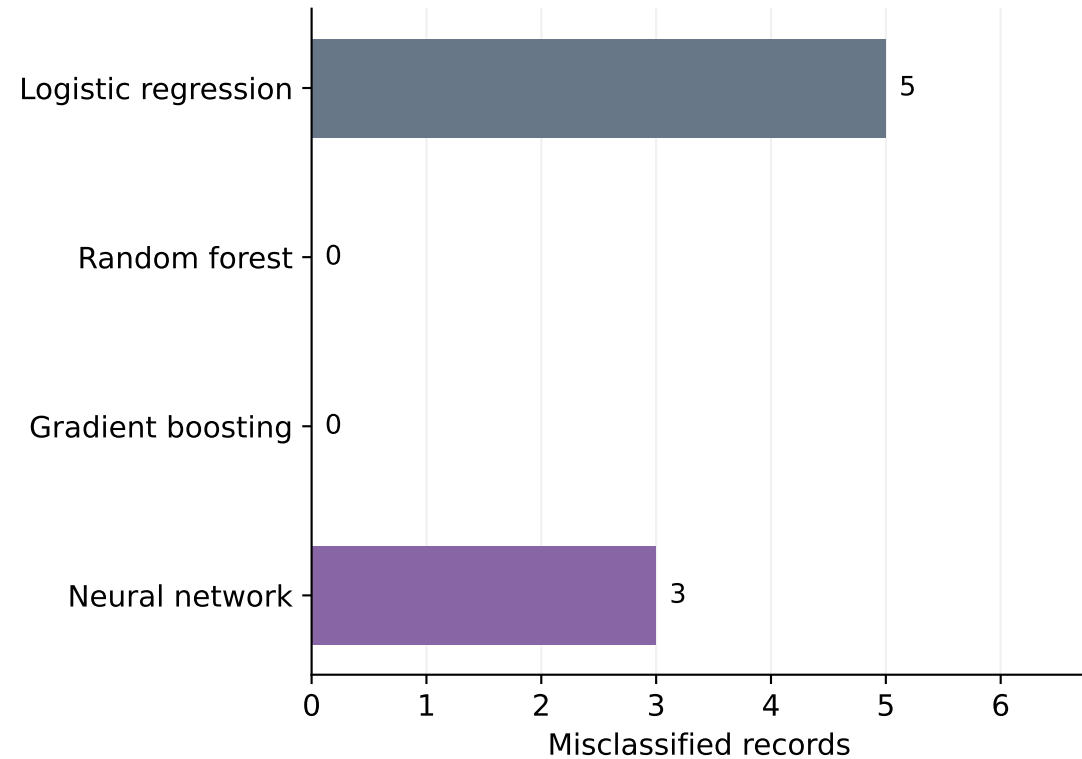
Test errors
