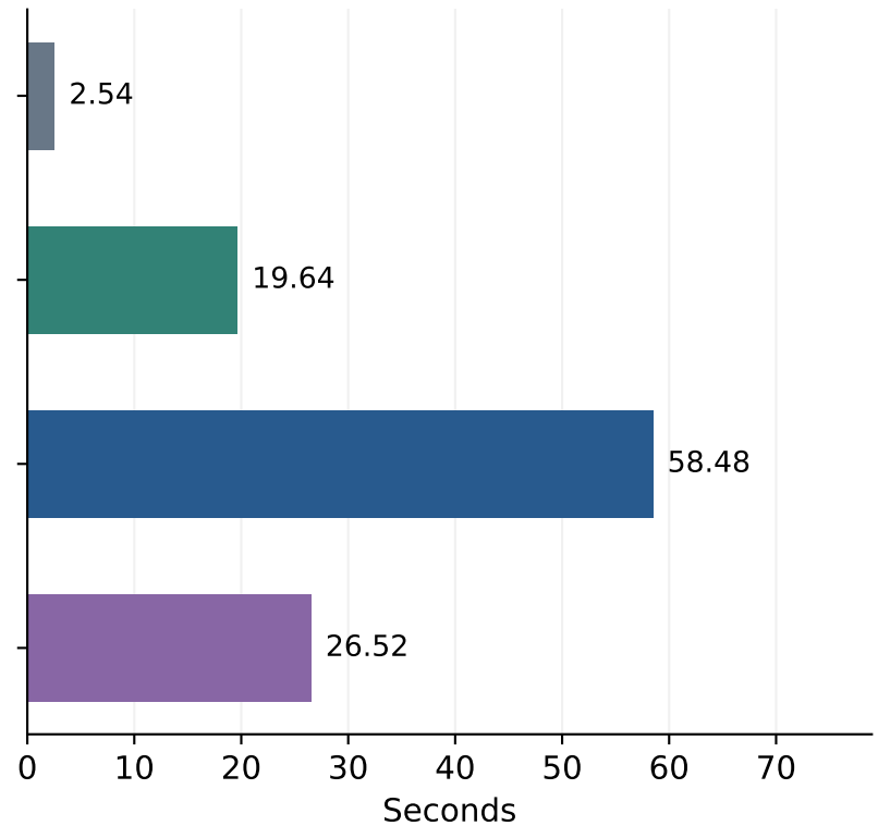
Training time
