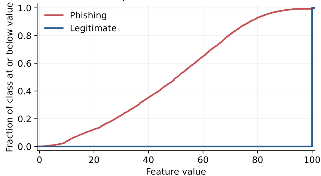
NoOfExternalRef Separation AUC = 0.9878
