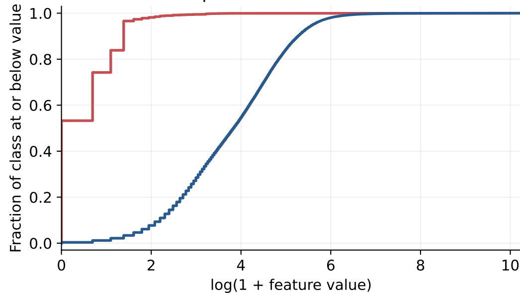
NoOfExternalRef Separation AUC = 0.9878
