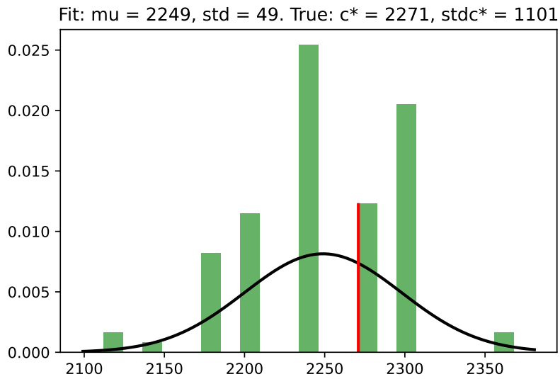
Figure 2: sandbox/approxmc-results/nopreproc/fuzzTest-44.c
