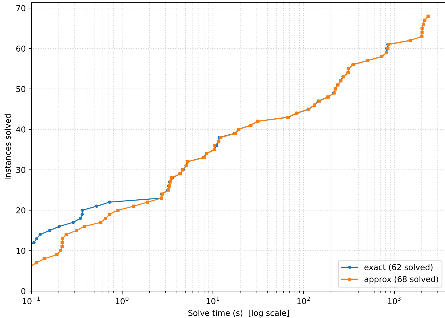
Ganak CDF - Track 1 private (exact vs approx)
