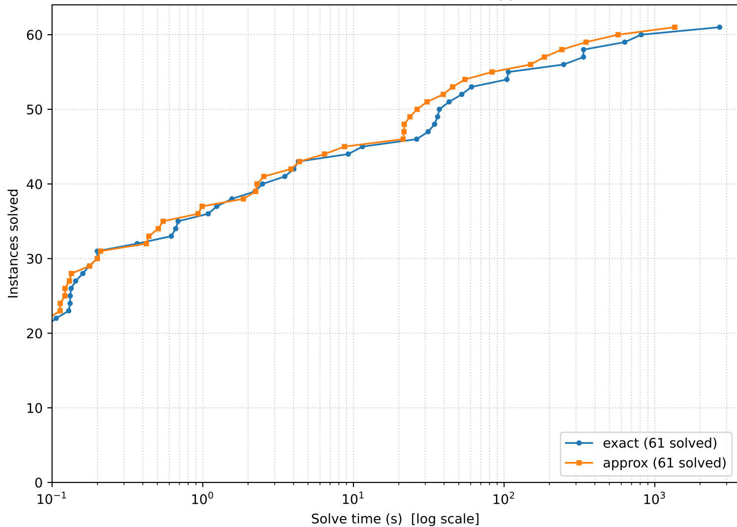
Ganak CDF - Track 2 (exact vs approx)
