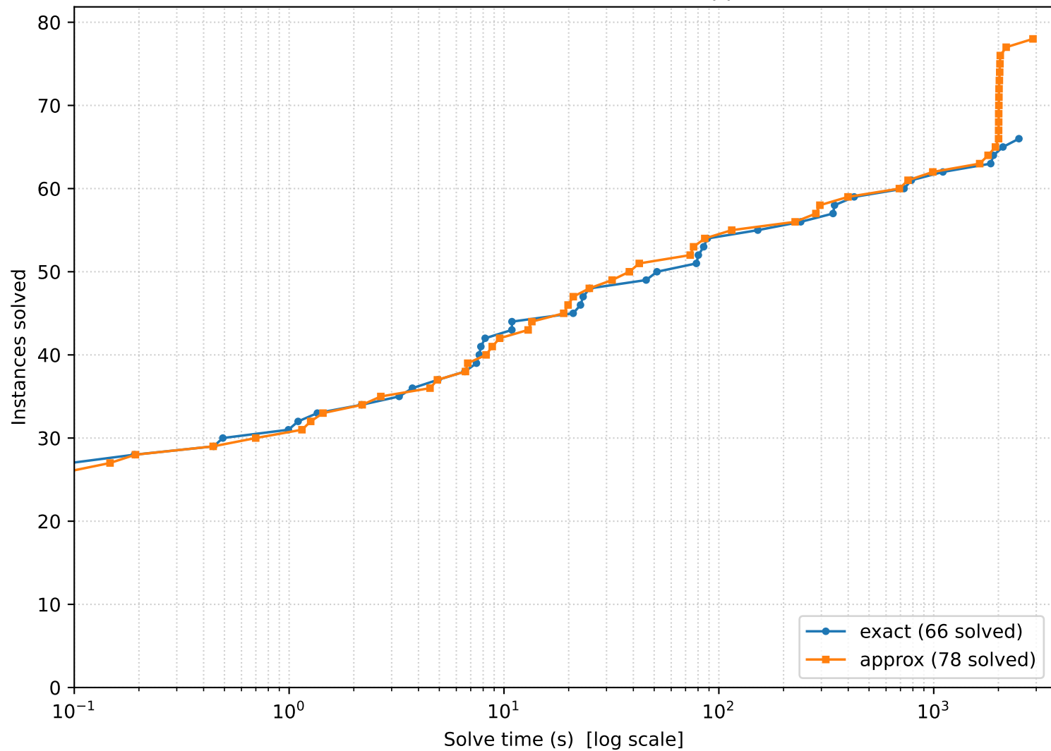
Ganak CDF - Track 4 (exact vs approx)
