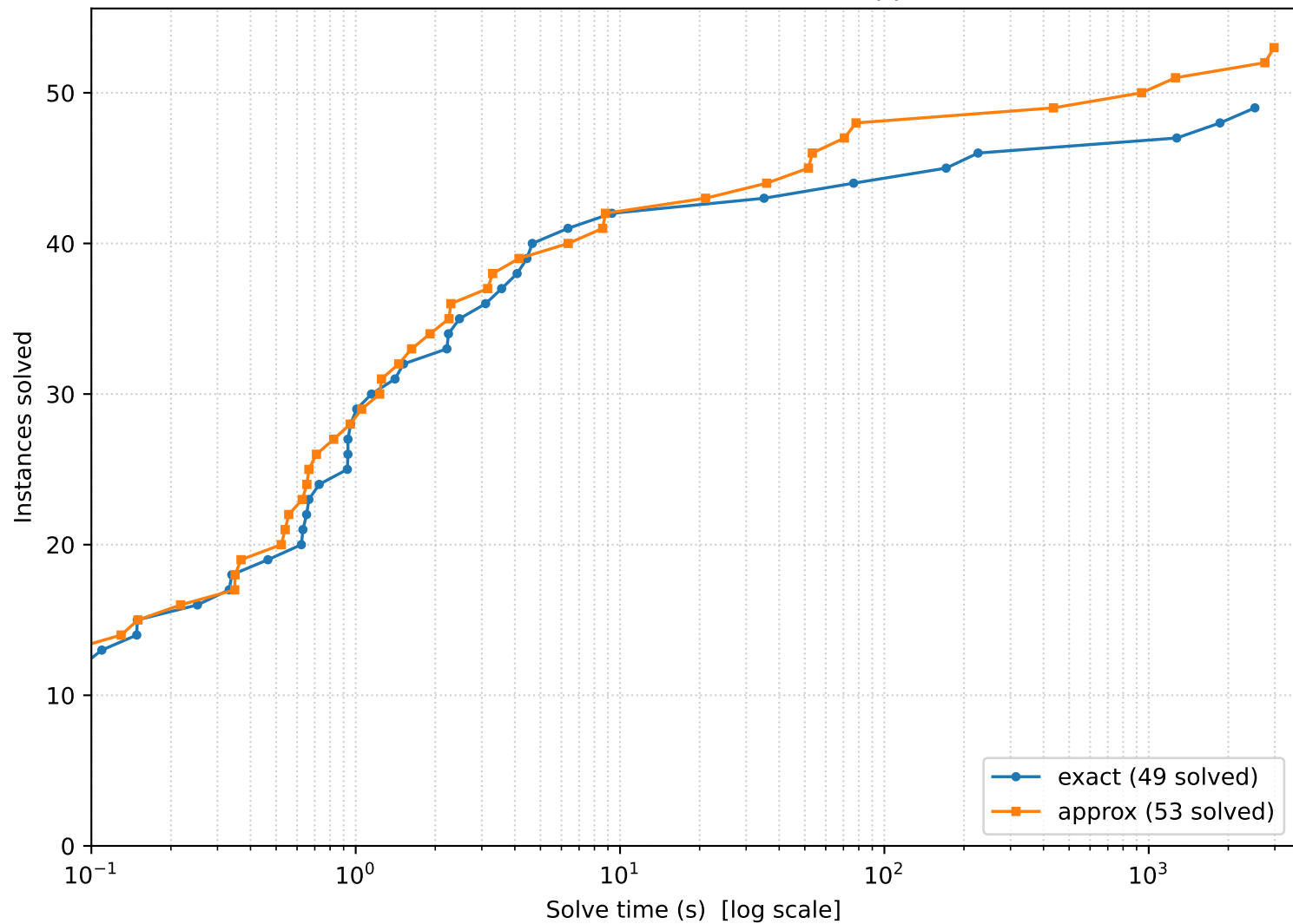
Ganak CDF - Track 5 (exact vs approx)
