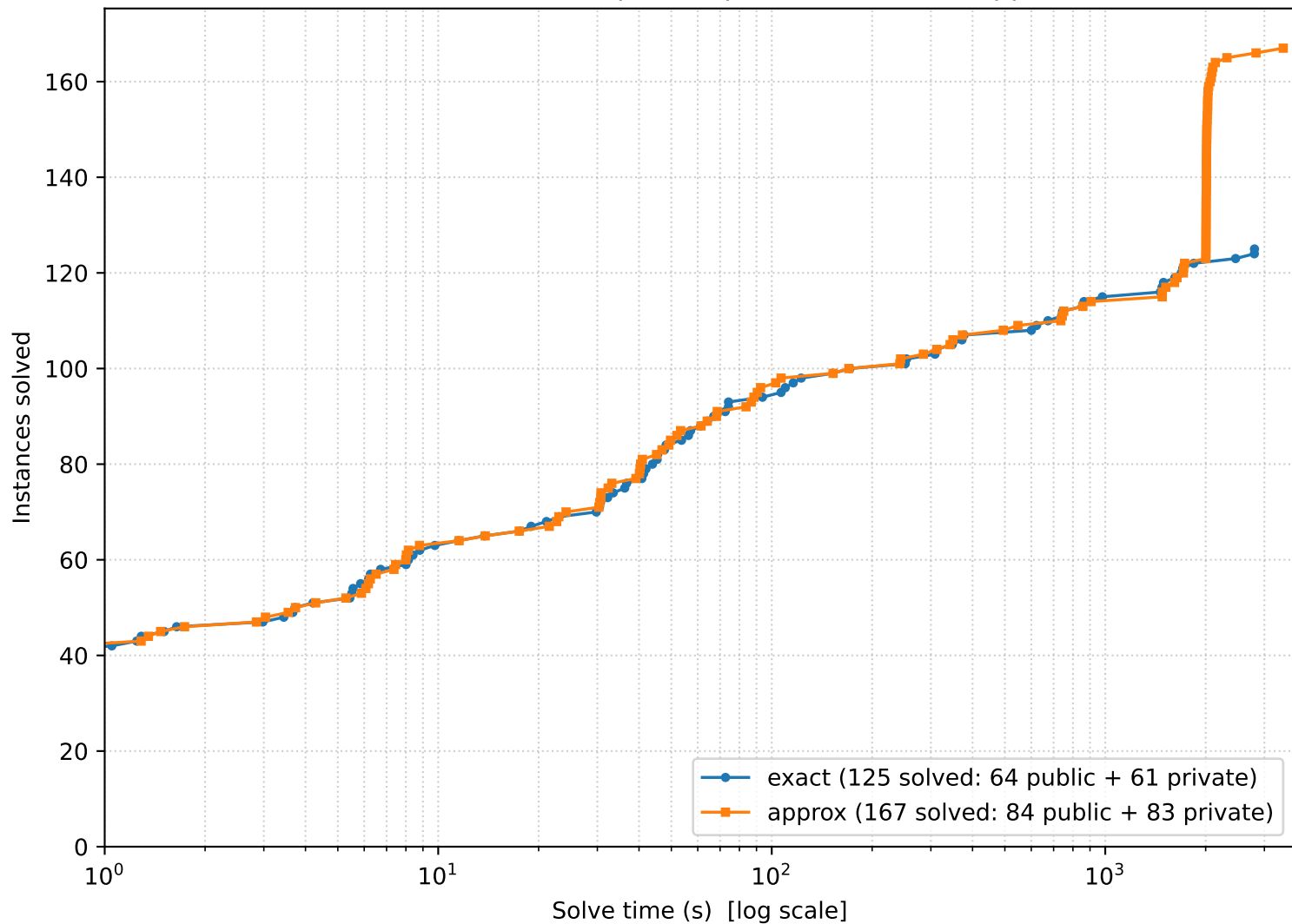
Ganak CDF - Track 3, public+private (exact vs approx)
