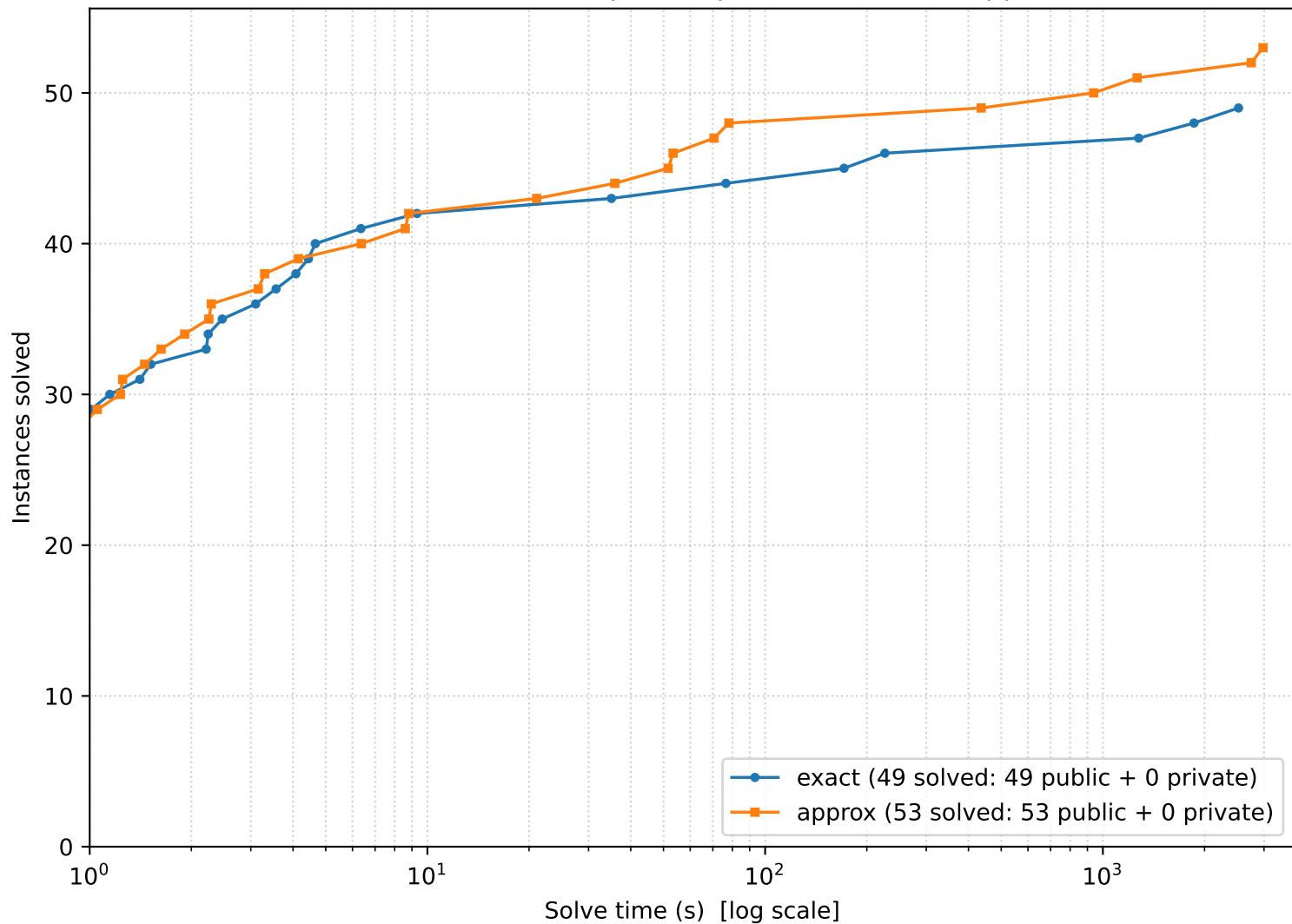
Ganak CDF - Track 5, public+private (exact vs approx)
