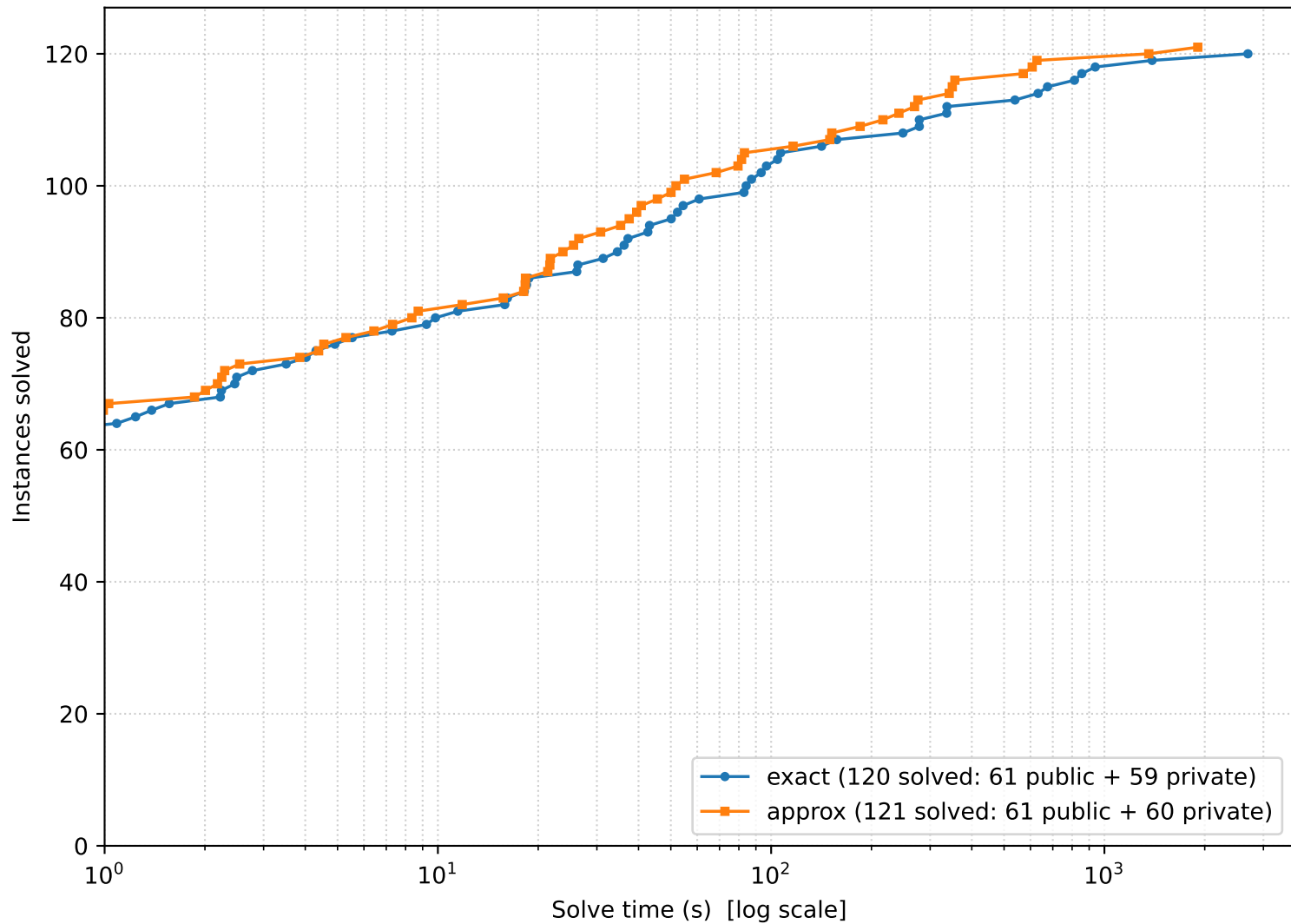
Ganak CDF - Track 2, public+private (exact vs approx)
