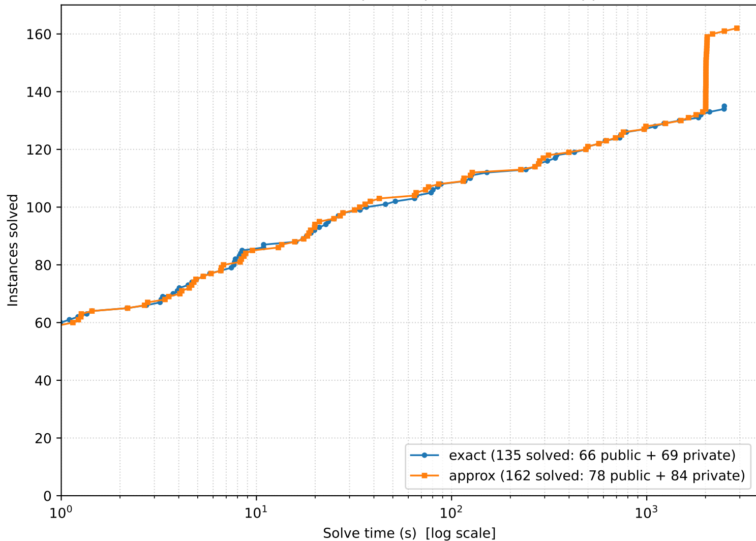
Ganak CDF - Track 4, public+private (exact vs approx)
