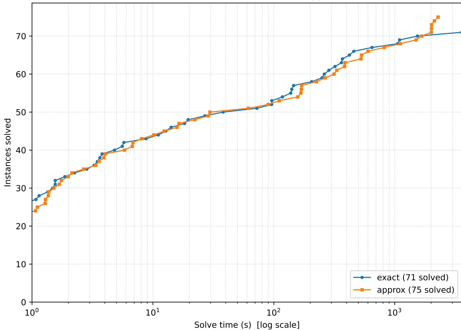
Ganak CDF - Track 1 (exact vs approx)
