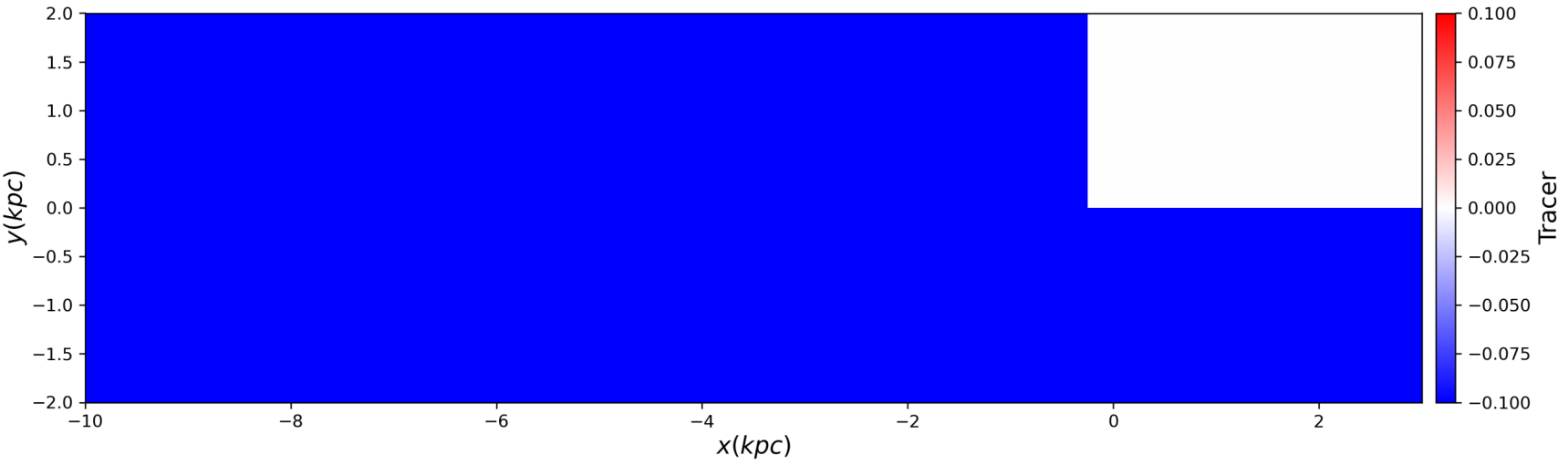
Outflow Tracer
