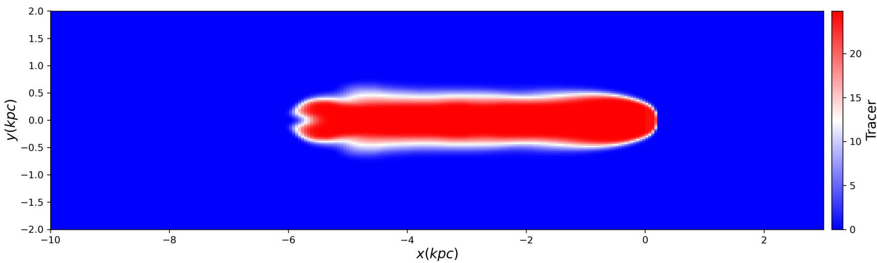
Outflow Tracer
