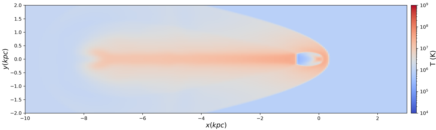
Temperature
