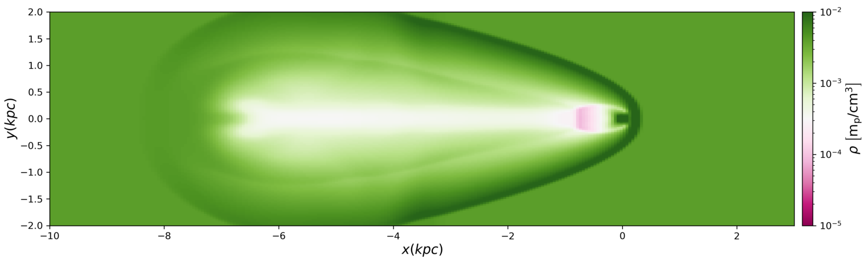
Density
