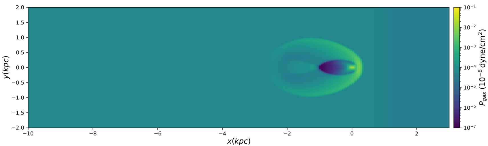
Pressure
