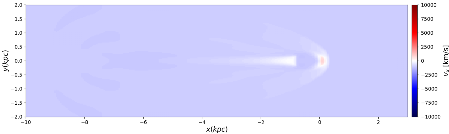
X Velocity
