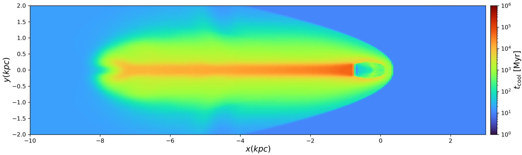
Cooling Time
