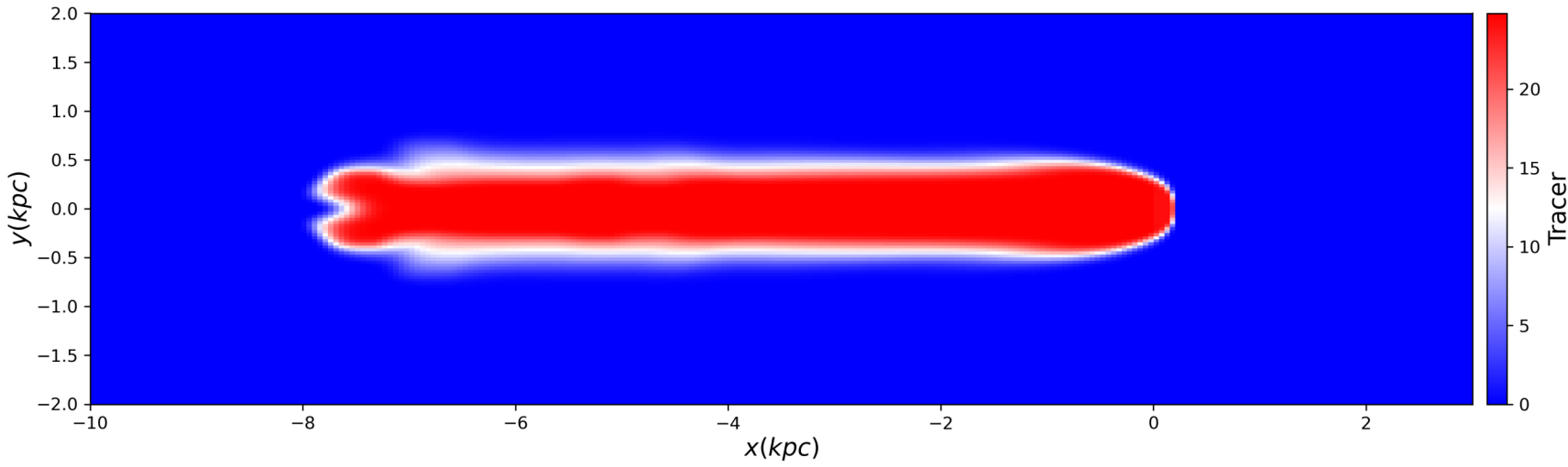
Outflow Tracer
