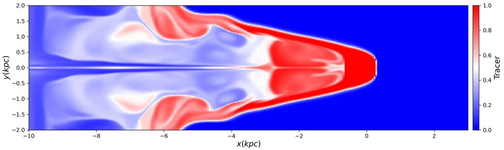
Outflow Tracer
