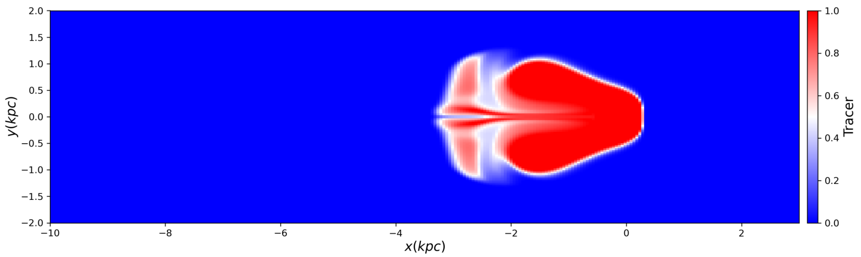
Outflow Tracer
