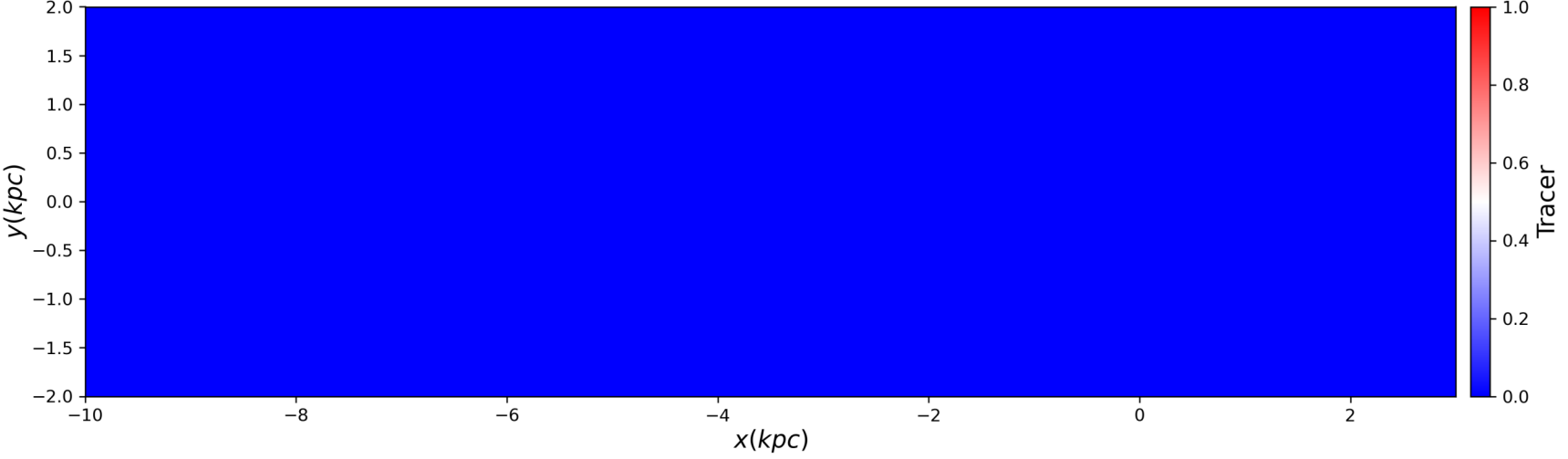
Outflow Tracer
