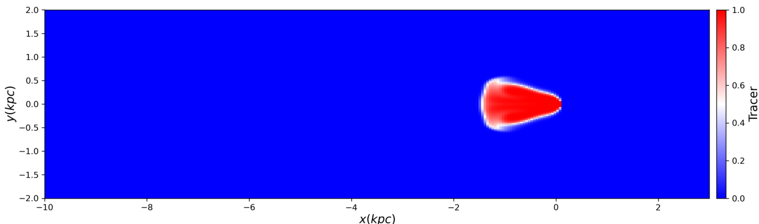
Outflow Tracer
