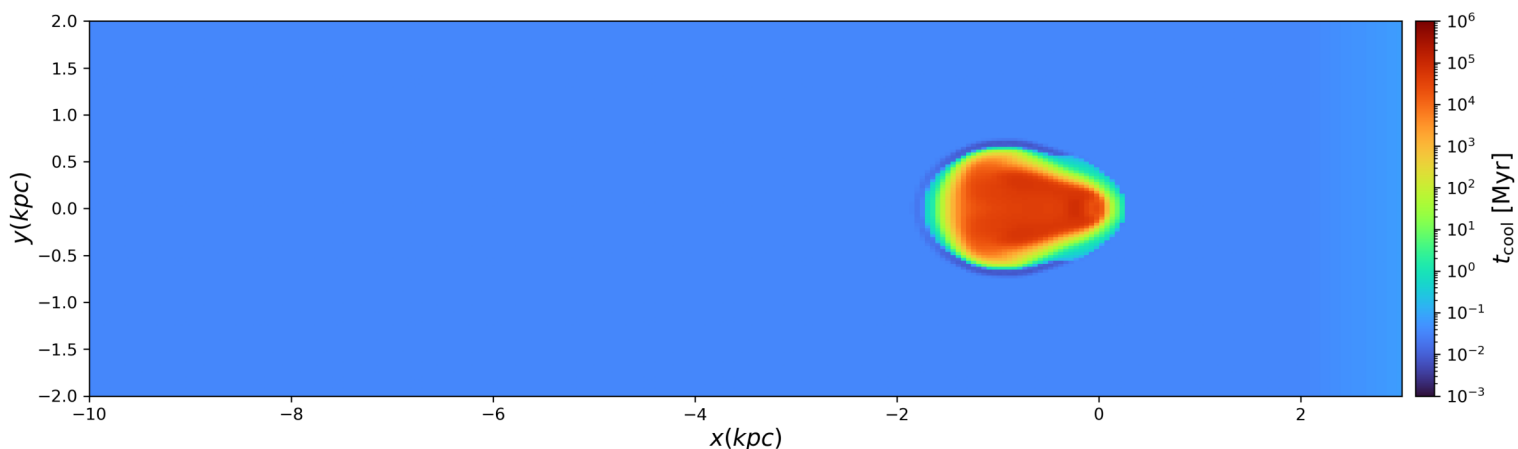
Cooling Time
