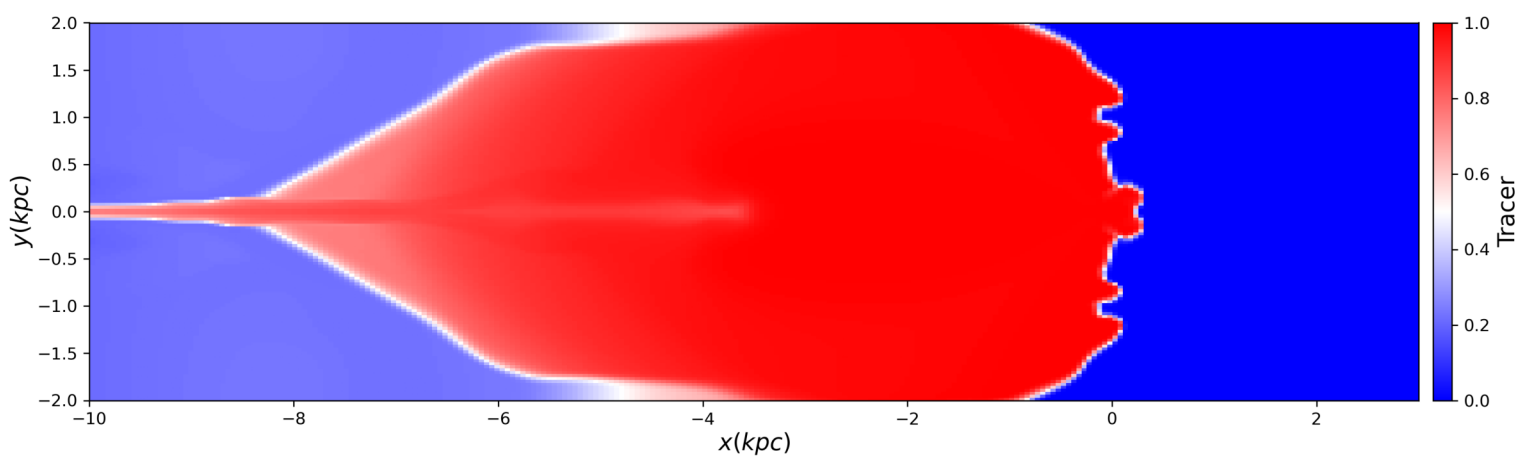
Outflow Tracer
