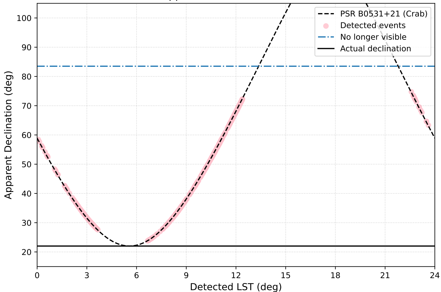
Apparent Declination vs. LST
