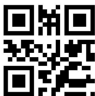
slof_306 ATOMS BOOK (Balaji S...
