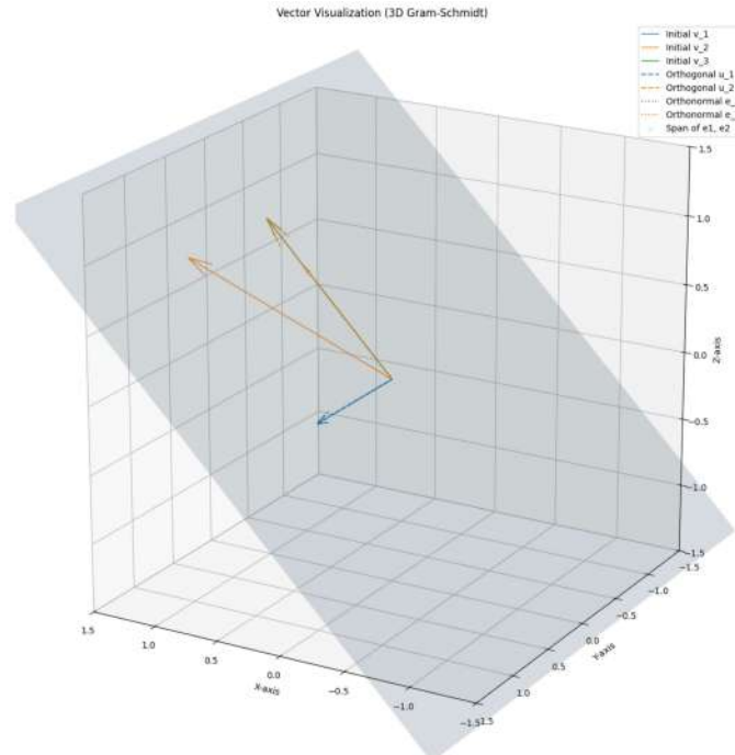
Figure 1: Orthonormalisation
