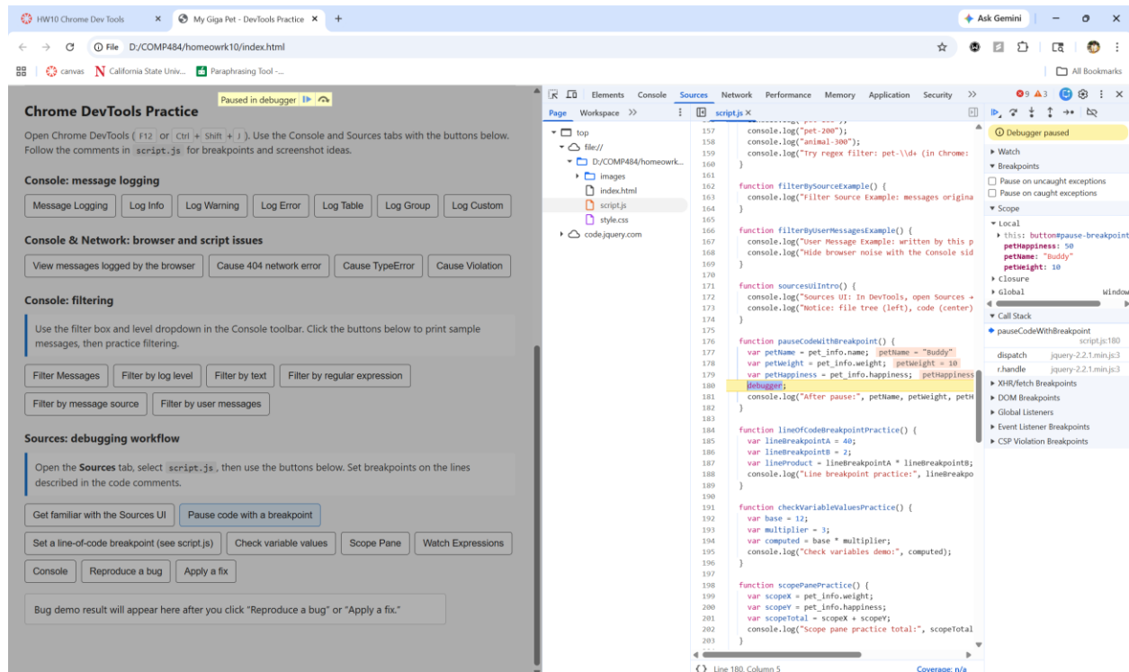
Figure 5 Sources: paused on breakpoint; Scope and Call Stack Screenshot: Execution paused on a debugger line; Scope (Local) and Call Stack visible.
