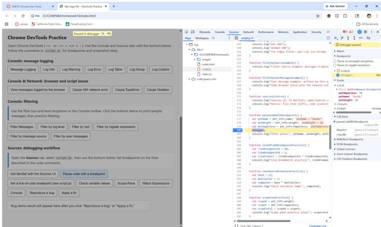
Figure 6 Sources: paused; Scope Screenshot: Second angle of paused state, or omit this figure in your final doc.
