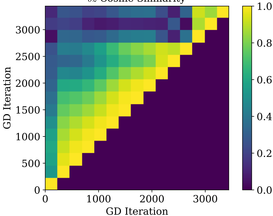
\delta z Cosine Similarity
