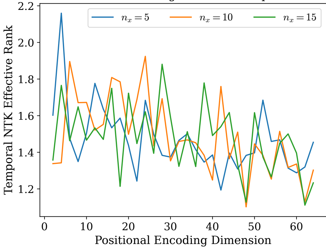
Vaswani Positional Encoding Increases Temporal NTK Rank
