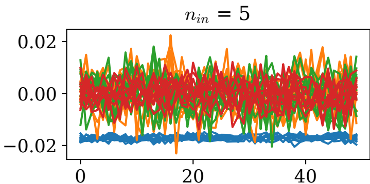
Weighted Temporal Modes
