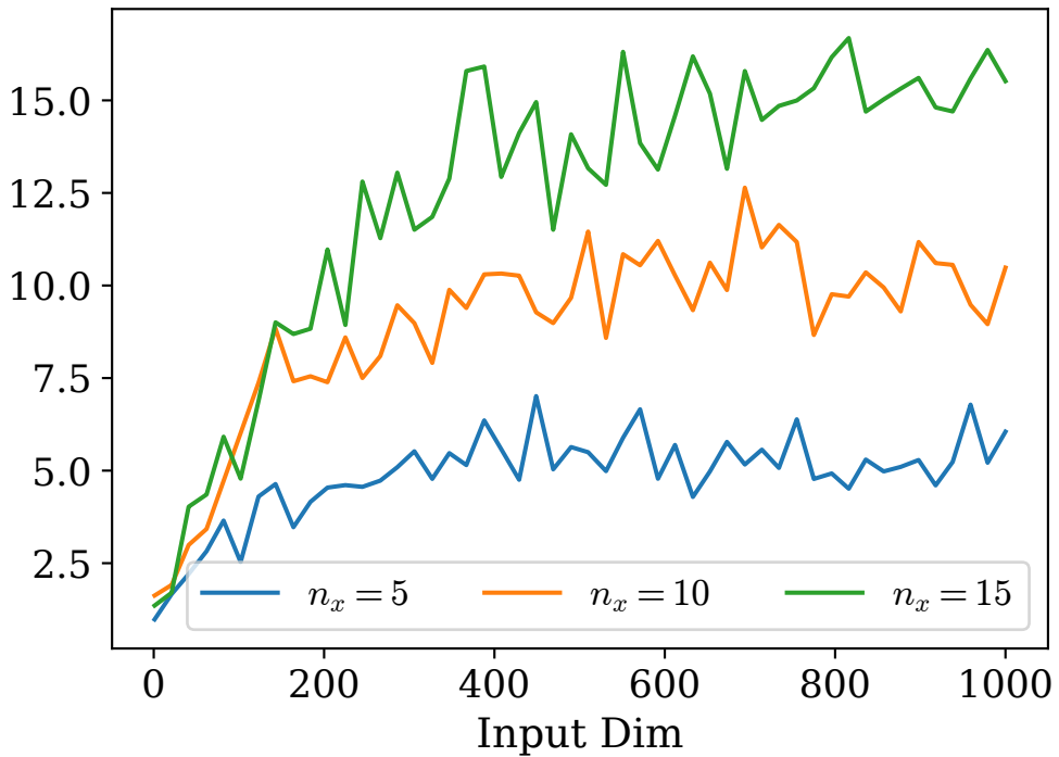
NTK Temporal Rank
